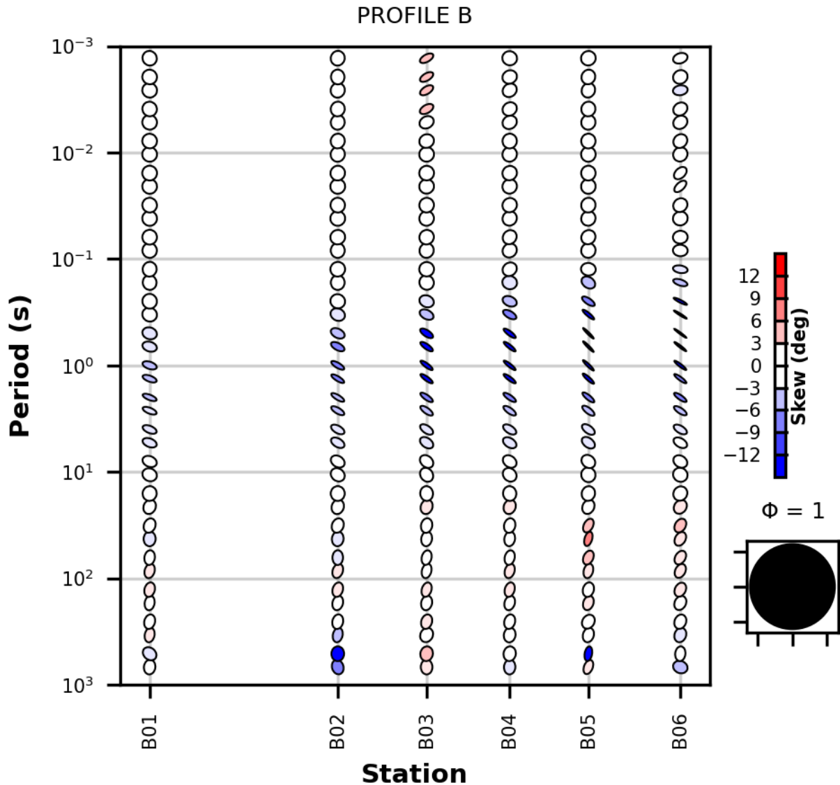
Figure 7. 7: Phase tensor pseudo-section plotted for all periods of MT data using MTPy (Kirkby et al., 2019; Krieger & Peacock, 2014): (a) profile A located south of the study area and showing 1-D structures at short periods and 3-D structure at long periods. (b) profile B located to the north in the study area and showing 1-D structures at periods less than 1 second. At long periods the data revealed a 3-D structure of the subsurface.
