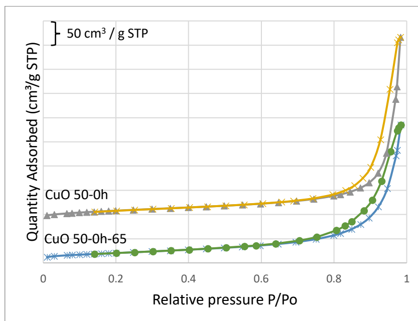
Figure 4.13 N 2 -physorption isotherms of the CuO 50-0h-65 and CuO 50-0h catalysts.
