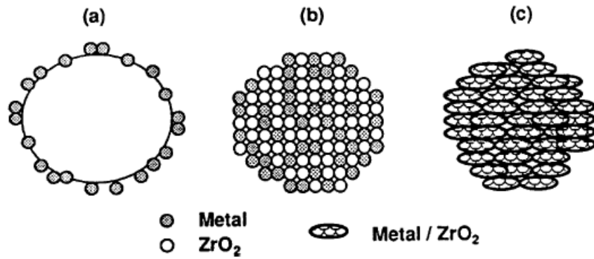
Figure 1.5 Structural features of catalysts prepared by different methods [7].
