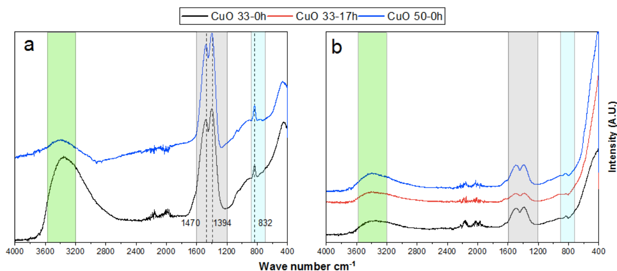
Figure 4.3 FT-IR spectra of the catalyst precursors (a) and the calcined catalysts (b).
