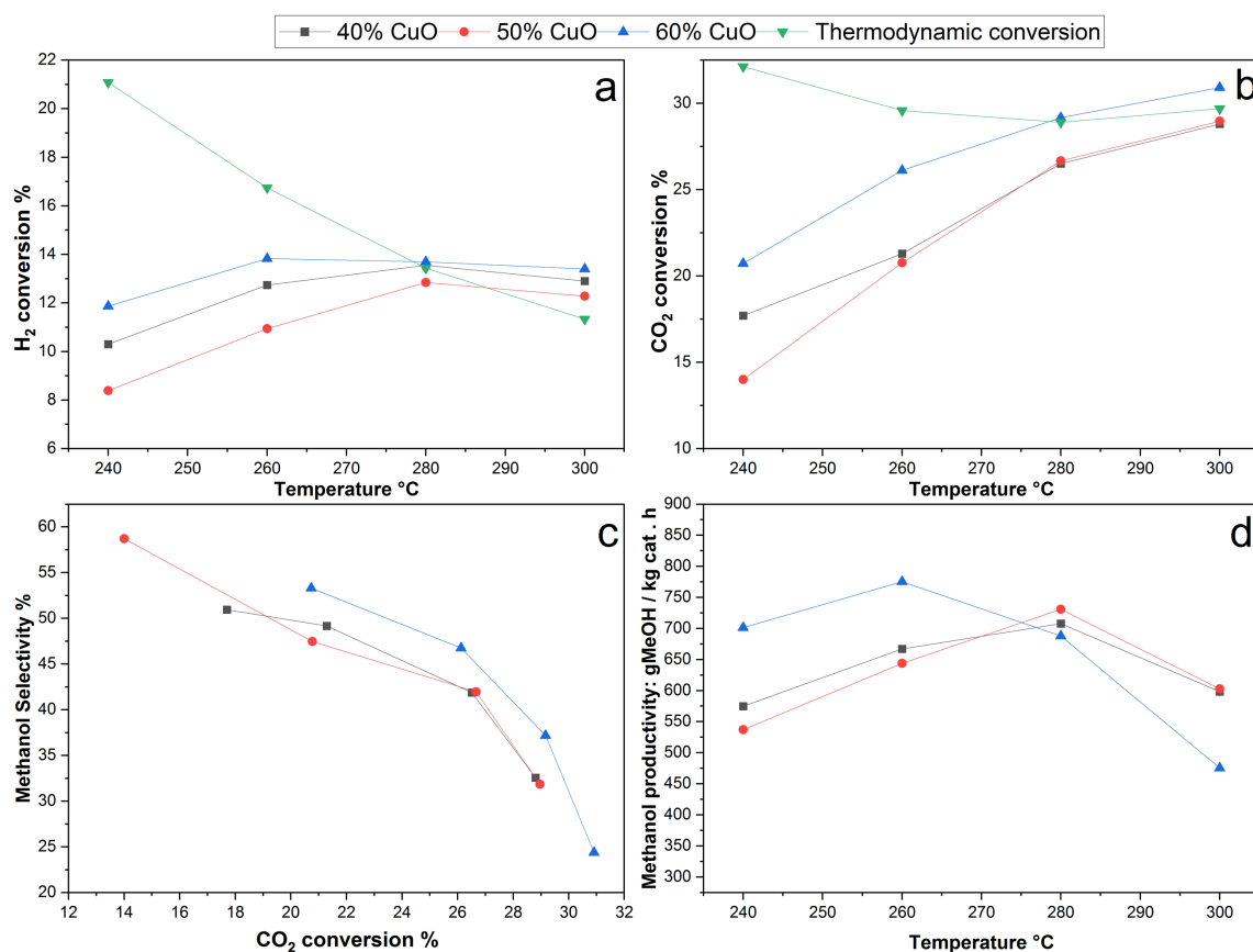
Figure 5.9 Catalytic performance of the catalysts 40% CuO, 50% CuO and 60% CuO. (a) H 2 conversion, (b) CO 2 conversion, (c) methanol selectivity against CO 2 conversion % and (d) methanol productivity. P: 50bar, GHSV: 24000Nml h -1 g -1 , molar ratio H 2 /CO 2 : 3.9.
