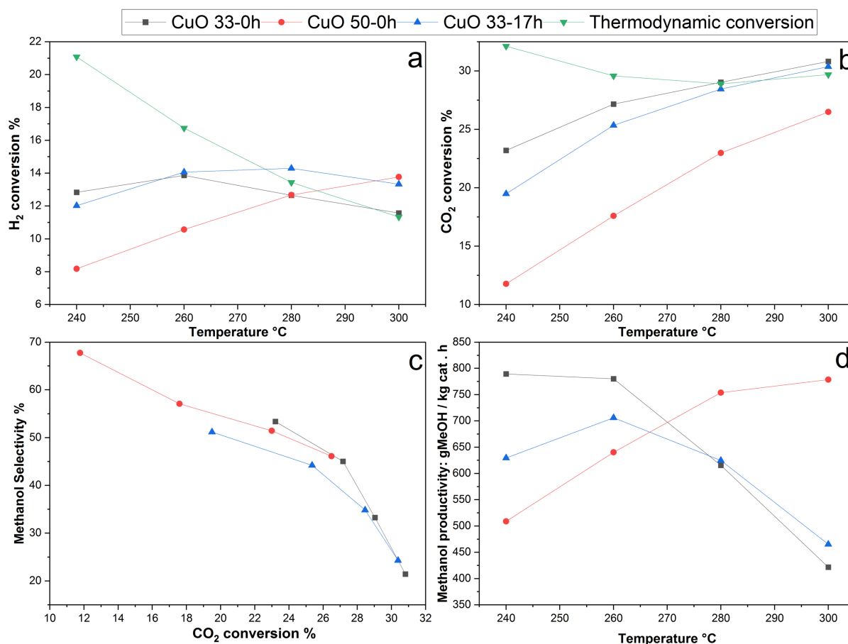
Figure 4.9 Catalytic performance of the catalysts under study. (a) H 2 conversion, (b) CO 2 conversion, (c) methanol selectivity and (d) methanol productivity. P: 50 bar, GHSV: 24000Nml h -1 g -1 , molar ratio H 2 /CO 2 : 3.9.
