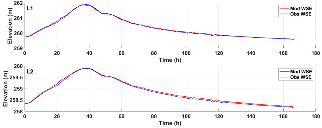
Figure 5.10: Comparison between the WSE recorded by the limnimeter L1 and L2, located on either side of the injection site, and the WSE modeled during the peak flood of period P_1 ( Q = 303m^3/s ), obtained from unsteady simulations performed using the submodel \mathcal{M}_{f,p} .
