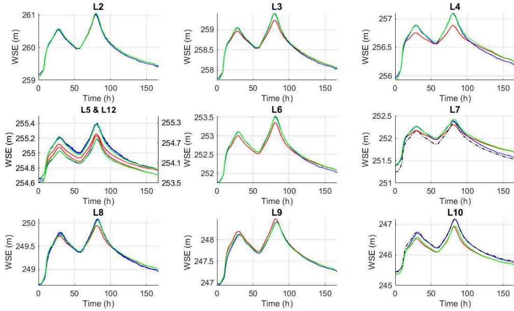
Figure 3.5: Comparison between observed and modelled WSE during the flood event F_1 (discharges ranging from 40 to 303m^3/s ). Blue solid line indicate the WSE recorded by the limnimeter L_n distributed along the Moselle river (Figure 3.1 D). Red and green solid line indicates the WSE modelled using the DEM of 2018, with a Strickler coefficient in the floodplain of 47m^{1/3}/s and 8m^{1/3}/s , respectively. Dashed black line indicates, at L7 and L10, the WSE modelled using the DEM of 2019 with a Strickler coefficient in the floodplain of 8m^{1/3}/s .
