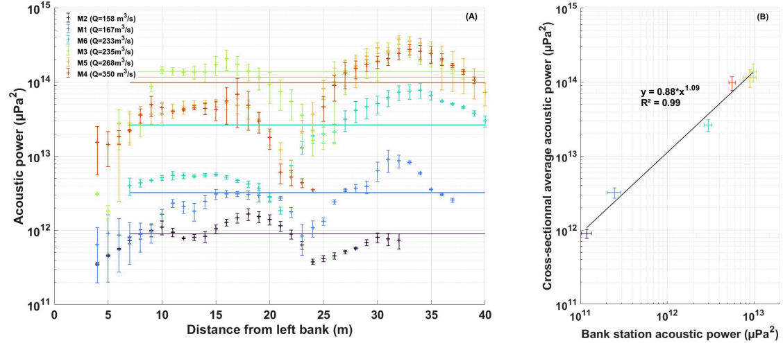
Figure 4.5: (A) Results of acoustics maps performed at different discharge and (B) relationship between bank and cross-section averaged measurements
