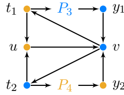
Figure 7.10: A 3-vertex u and its lonely neighbour v in a dicolouring \phi from which we cannot reach the dicolouring \psi swapping the colours of u and v via a redicolouring sequence. Vertices coloured 1 are shown in orange, while vertices coloured 2 are shown in blue. Vertex t_1 must be blocked, yielding the existence of monochromatic path P_3 and the arc vt_1 . Vertex v must be blocked after recolouring t_2 , yielding P_4 and the arc vt_2 .
