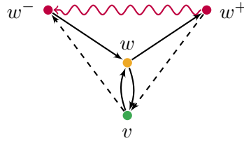
Figure 7.6: The vertices v, w, w^+ and w^- .
