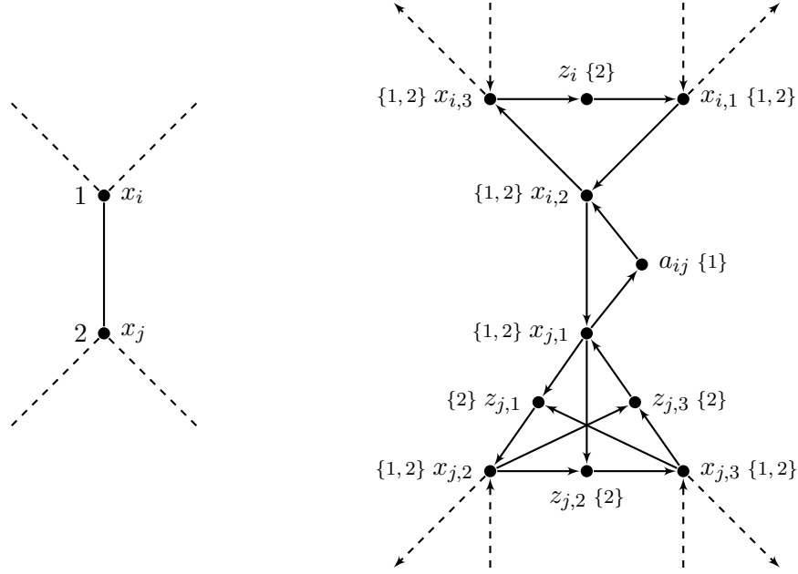
Figure 7.1: An example of building (D, L) from (G, \phi) , where \phi(x_i) = 1 , \phi(x_j) = 2 , and i < j .
