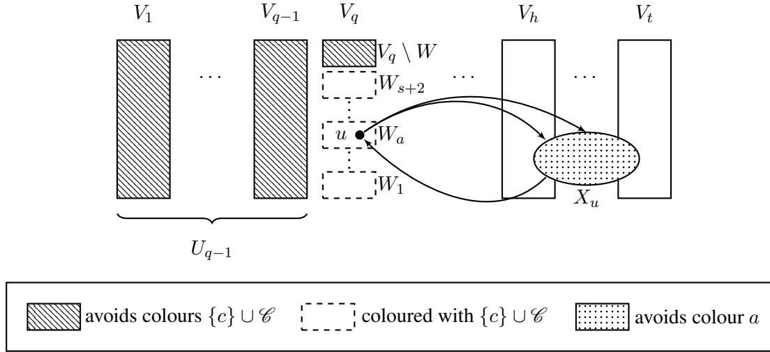
Figure 7.4: The structure of the digraph D dicoloured with \alpha , which we assume to be an (s+2) -dicolouring for clarity. Note that W_c does not exist and X_u may intersect V_{q+1} \cup \dots \cup V_{h-1} .
