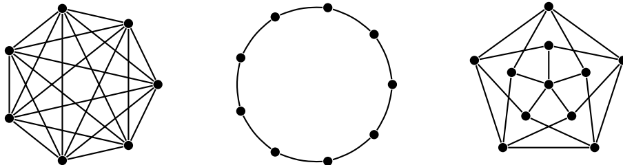
Figure 1.1: Examples of graphs. From left to right: the complete graph on 7 vertices, the cycle on 9 vertices, and the Grötzsch graph.
