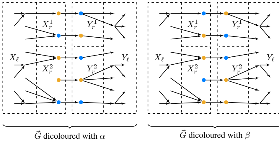
Figure 7.7: The partitioning of V(\vec{G}) into X_r^1, X_r^2, X_\ell, Y_r^1, Y_r^2, Y_\ell .
