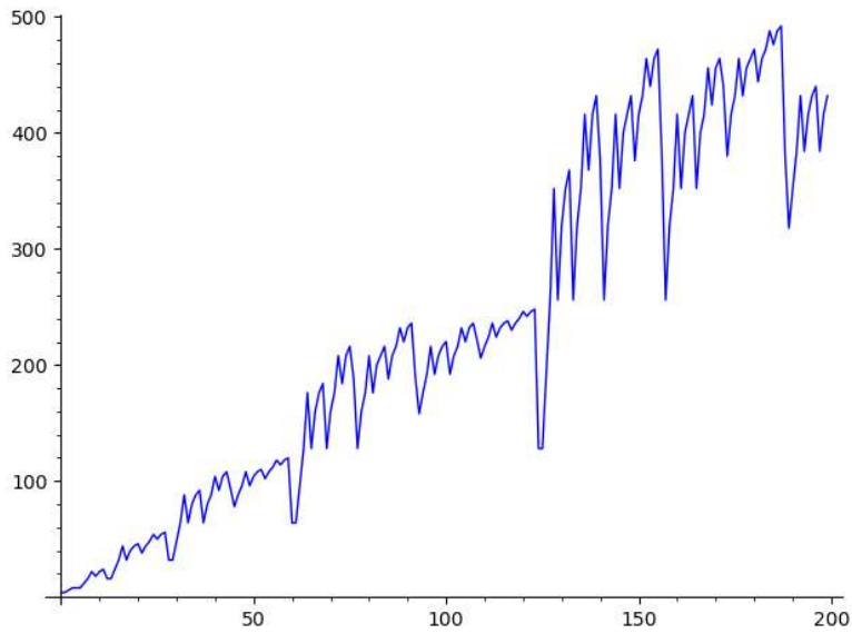
Figure 1: The values of Z(s) for 1 \leq s \leq 200 .
