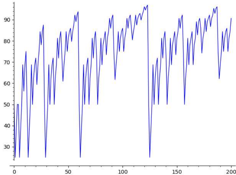
Figure 2: The values of \frac{Z(s)}{p(v^s)} for 1 \leq s \leq 200 .
