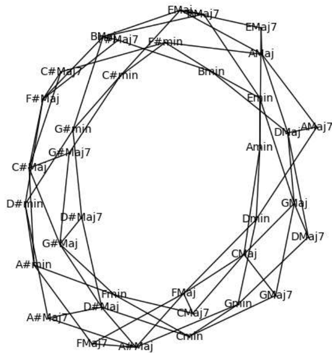
Figure 4.2: The graph of chords G .
