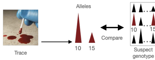
Figure 5.4: DNA individualisation
