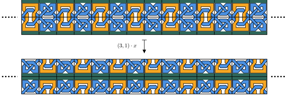
Figure 1.1: A configuration x from the full-shift over the alphabet A = \{\text{blue square}, \text{orange square}, \text{blue square}, \text{orange square}\} and group G = \mathbb{Z} \times \mathbb{Z}/2\mathbb{Z} , as well as its shift by g = (3, 1) . The configuration is inspired by the frieze patterns at the Alhambra [Bod07].
