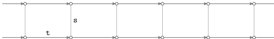
Figure 1.12: A Cayley graph of the group \mathbb{Z} \times \mathbb{Z}/2\mathbb{Z} . The generator t defines the horizontal right-pointing edges, and the generator s defines the vertical undirected edges.
