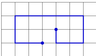
Figure 4.2: On \mathbb{Z}^2 with standard generating set: a finite SAW that does not appear in a bi-infinite SAW.
