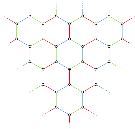
Figure 1.11: A Cayley graph of the affine Coxeter group \tilde{A}_2 . The red edges represent a , blue edges represent b , and green edges represent c .
