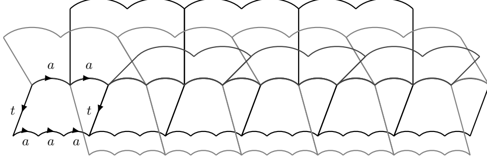
Figure 6.6: The Cayley graph of BS(2, 3) = \langle a, t \mid t^{-1}a^2t = a^3 \rangle
