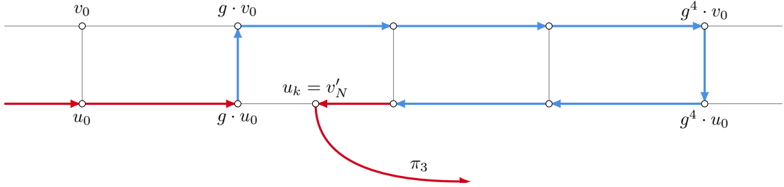
Figure 4.7: The periodic subdivision of the 2-ladder with the configuration x highlighted in red and blue. The word \lambda_2 \lambda_3^3 \lambda_2^{-1} \lambda_1^{-2} is marked in blue, whereas the infinite prefix and suffix of x are marked in red.
