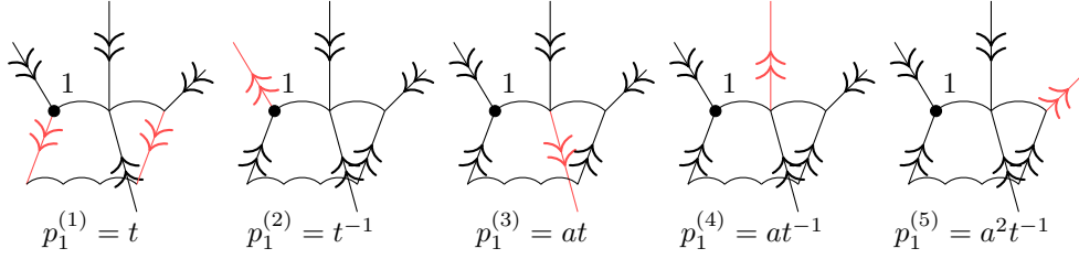
Figure 6.8: The allowed patterns p_1^{(1)} to p_1^{(5)} for the flow SFT on BS(2,3) . For more readability the outgoing edges are pictured in red.
