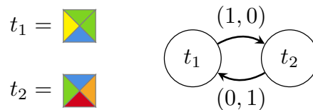
Figure 1.8: An example of the tileset graph obtained from two Wang tiles t_1 and t_2 . Inverses of the generators for \mathbb{Z}^2 are omitted for simplicity
