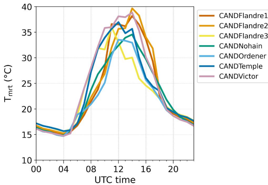
Figure 68: Average daily evolution of the mean radiant temperature ( T_{mrt} ) calculated at each lamp post from May 1 st , 2021 to September 30 th , 2021. T_{mrt} was not calculated at Paris-Montsouris. Standard deviation is not represented for more clarity but can reach 13.9 °C.
