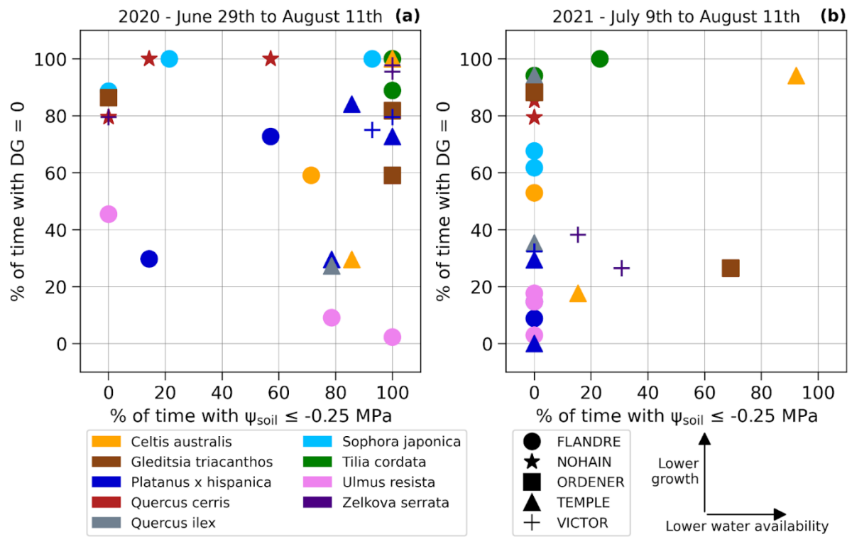
Figure 86: Percentage of time without growth of the studied branches as a function of the percentage of time with soil water potential \Psi_{soil} lower than the measurement range of the probes (-0.25 MPa) for the 36 studied trees during summer 2020 ( (a) from June 29 th to August 11 th ) and 2021 ( (b) from July 9 th to August 11 th ).
