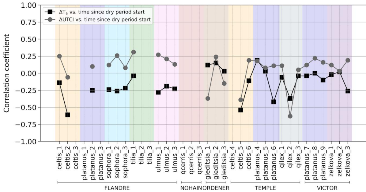
Figure 89: For each tree, correlation coefficient between the daily air temperature difference ( \Delta T_a , tree - lamp post) and daily UTCI difference ( \Delta UTCI , tree - lamp post) with the progress of the studied dry period for days sunny (more than 10 hours of insolation) and rain-free days from July 1 st to August 10 th 2020.
