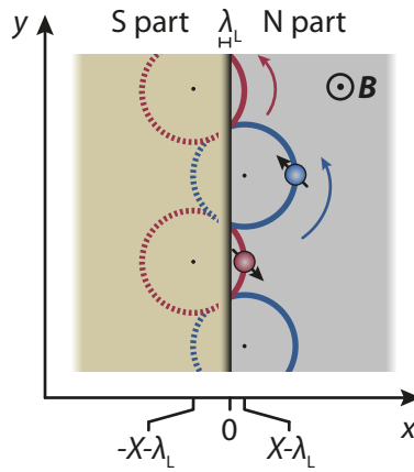
Figure 1.6: NS interface in the quantum Hall regime. The boundary between the superconducting lead and the 2DEG in the quantum Hall regime locates at x = 0 . In the semiclassical picture, a proximitized quantum Hall edge state can be viewed as successive Andreev reflections along the interface. Note that as an Andreev-reflected hole (color-coded in red) undergoes both effective mass and charge sign reversals, its cyclotron motion is directed towards the same direction as the electrons (color-coded in blue). The London penetration depth \lambda_L shifts the guiding center coordinate X of these cyclotron orbits towards the superconducting electrode.
