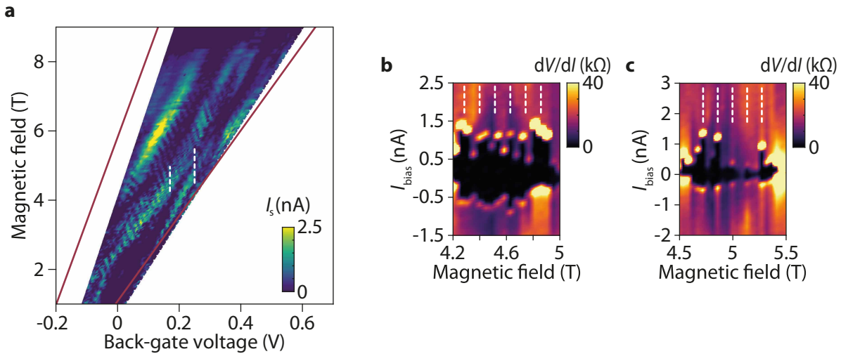
Figure 5.1: Switching current oscillations across the V_g - B . a) Switching current I_s colormap versus both the back-gate voltage V_g and the magnetic field B obtained at T = 10 \text{ mK} for narrow junction B ( L \times W = 140 \times 177.5 \text{ nm}^2 ) in sample HV088. Red lines indicate the \nu = 2 QH plateau's edges measured at I_{\text{bias}} = 160 \text{ nA} . b) Colormap of the differential resistance dV/dI versus the magnetic field B and the current bias I_{\text{bias}} computed from the successive I/V characteristics done along the leftmost white dashed line in (a) , i.e. at V_g = 0.17 \text{ V} . Periodicity of the overlying white comb is 114.8 \text{ mT} , a value that falls within the window of magnetic field period values compatible with the h/2e -flux periodicity (i.e. from 63 \text{ mT} to 122 \text{ mT} , see Appendix B for uncertainty on the area estimation). c) Colormap of the differential resistance dV/dI versus the magnetic field B and the current bias I_{\text{bias}} computed from the successive I/V characteristics done along the rightmost white dashed line in (a) , i.e. at V_g = 0.25 \text{ V} . Periodicity of the overlying white comb is 137.8 \text{ mT} , a value that falls within the window of magnetic field period values compatible with the h/e -flux periodicity ( 125 \text{ mT} to 243 \text{ mT} ).
