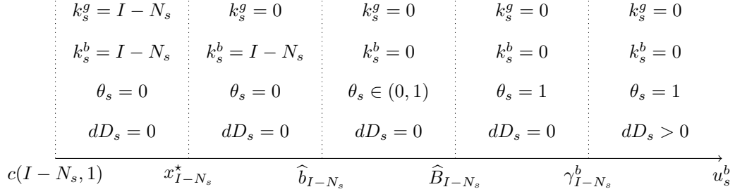
Figure 3.2: Optimal contract on the upper boundary.
