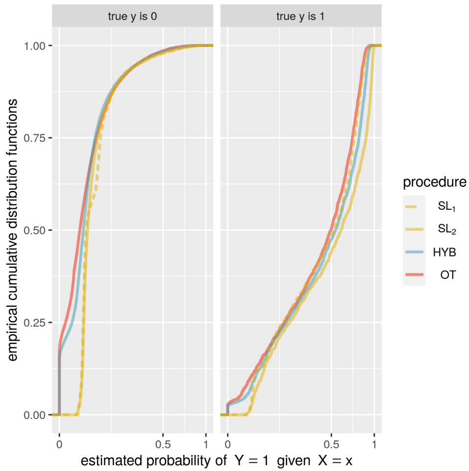
Figure 4.1: Empirical cumulative distribution functions of the sets \{\hat{y}_{n,\ell}^\bullet : \ell \in \llbracket L \rrbracket, n \in \llbracket N \rrbracket \text{ st } y'_{n,\ell} = y\} for y = 0 (left-hand side panel) and y = 1 (right-hand side panel), where the symbol \bullet stands for SL_1, SL_2, OT, HYB .
