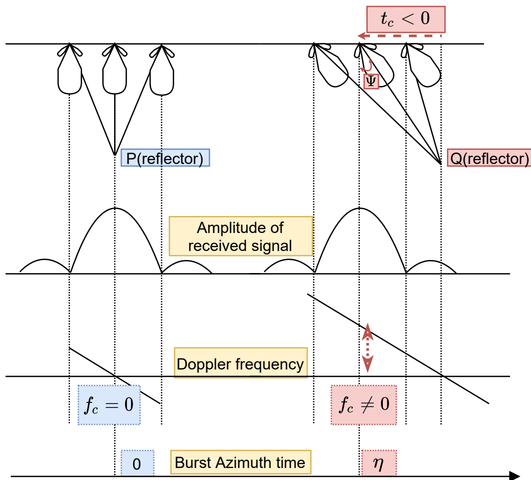
Figure 3.1: Downward view of the slant range plane during a TOPSAR burst acquisition. On the left, in blue, the antenna beam is orthogonal to the trajectory (near the middle of the burst). The Doppler frequency at the point of maximum amplitude is 0 Hz. On the right, in red, at azimuth time \eta , the beam has a squint angle \Psi w.r.t. the zero Doppler plane. The point of max amplitude is reached earlier, and the Doppler frequency at this position is not null and is proportional to the radial velocity component (projection on line of sight)
