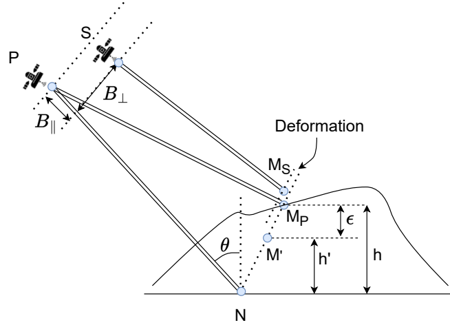
Figure 1.3: Differential Interferometry (DInSAR) principle. The scene is acquired from a satellite at two positions P (Primary) and S (Secondary), corresponding to two passes at different dates along the same orbit. Between the two dates, the target moved from position M_P to position M_S . The scale of the figure is inaccurate for visualization purposes: the deformation (millimetric) is actually many orders of magnitude smaller than the satellite-target distance (hundreds of kilometers) and the topography (meters, depending on the terrain). The figure shows as well point N, which would have been acquired in the same range sampling cell in the absence of topography on the reference surface. Also, point M' is the location of point M given by an external data source, such as DEM. The assumed height h' of M' has an error w.r.t. the true height h of \epsilon . The geometric baselines B_\perp and B_\parallel and the incidence angle \theta are also represented.
