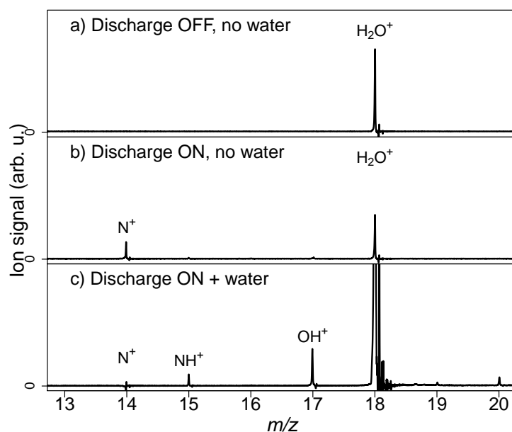
Figure 2.16: Mass spectra recorded for reaction of \text{H}_2\text{O} with N produced by discharge from 6% \text{N}_2 in He, at the photon energy of 13.519 eV. a) No discharge voltage is applied, and no water is injected. b) High discharge voltage is applied, without the injection of water. c) High discharge voltage and continuous water vapor are supplied.
