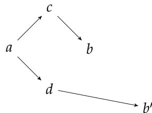
Figure 3.9 – Forking
