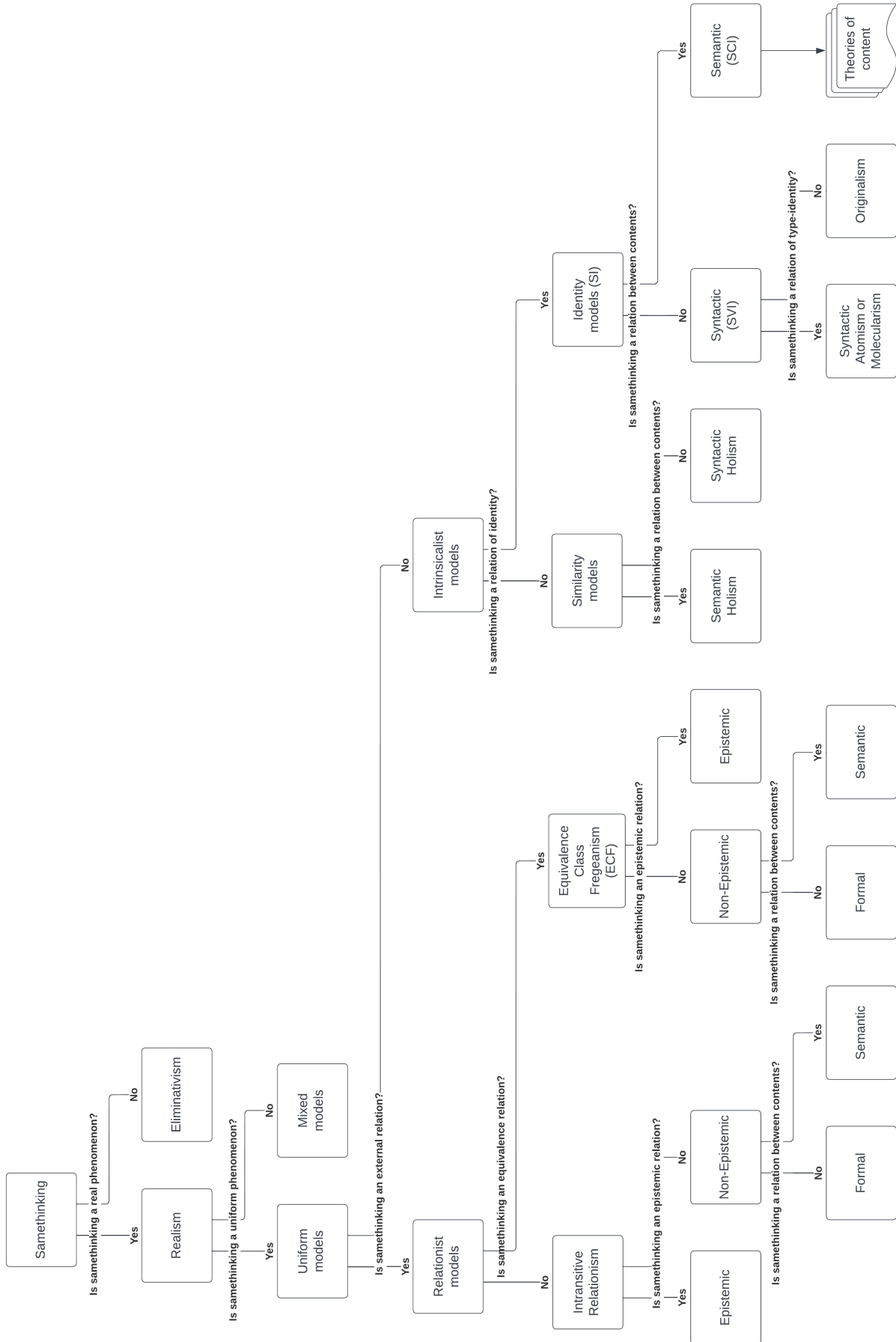
Figure 6.1 – Solution space
