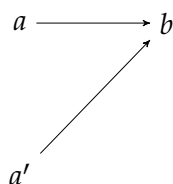
Figure 3.10 – Pooling (1)
