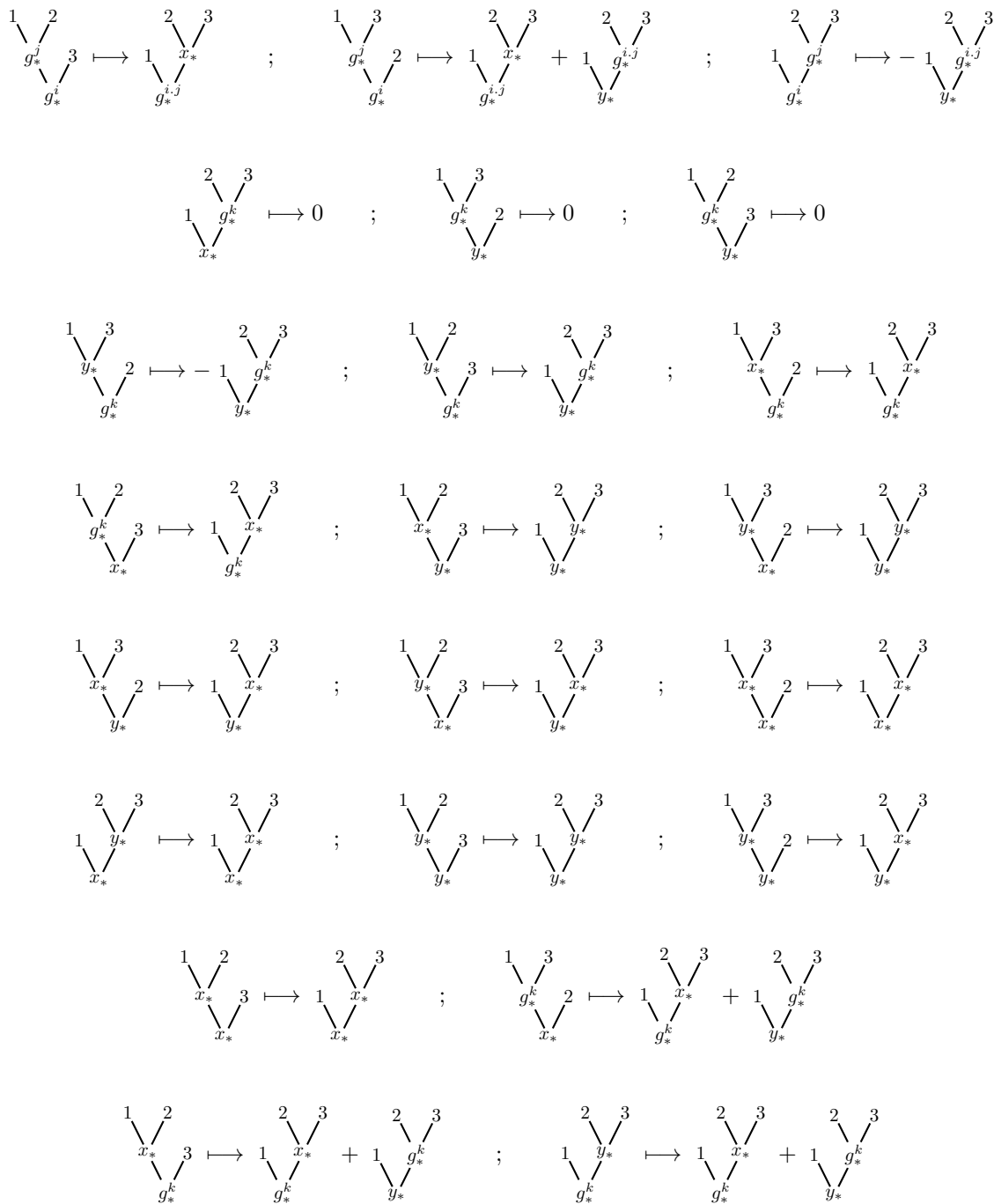
Figure 4.11: The “gplp” rewriting system for (\mathcal{G}^C)! .
