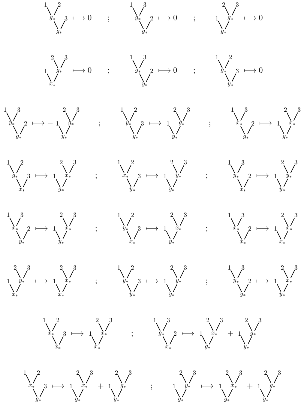
Figure 4.7: The “dp” rewriting system for (\text{Greg}')^! .
