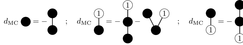
Figure 3.2: Composition of the arity 1 degree 1 elements.
