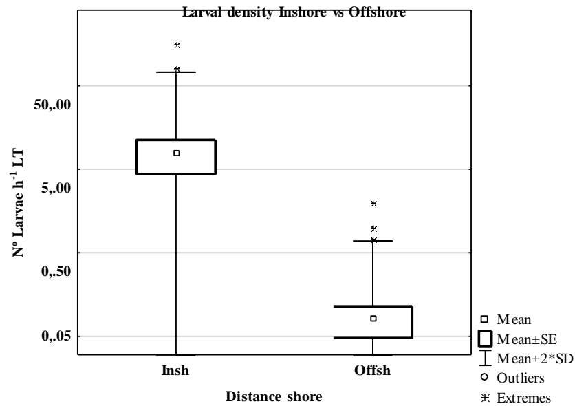
Figure 3.6: Box plots of larval density for the light trap samples collected in the inshore and offshore waters.
