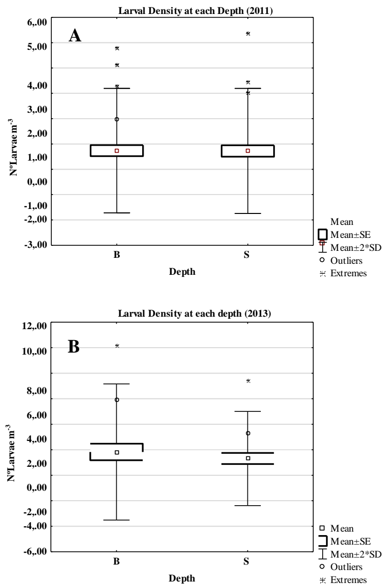
Figure 3.5. Box plots of larval density at the surface and bottom for scooter samples in (A) 2011 and (B) 2013.
