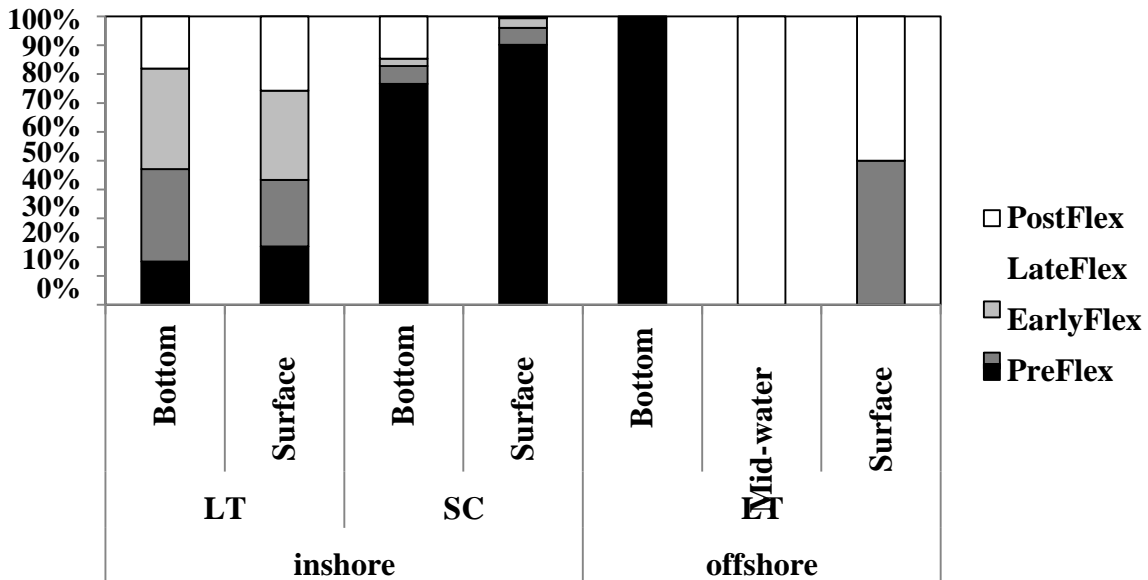
Figure 3.10 Bar plot showing ontogenetic differences between light trap and scooter samples.
