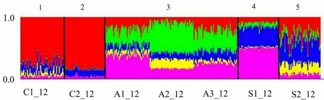
Figure 2.4. STRUCTURE Bar Plot for the “adult” data set, k = 5
