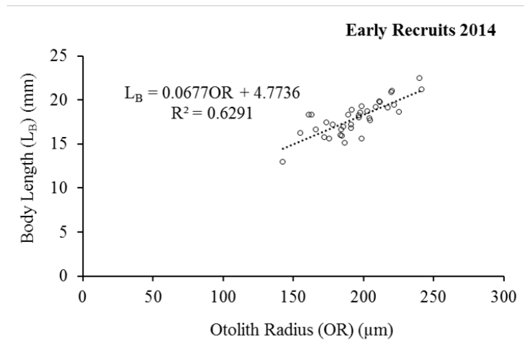
Figure 5.3 Relationship between body length ( L_B ; mm) and otolith radius (OR; \mu\text{m} ) for larvae caught in (B) 2013, and (C) early recruit samples caught in 2014. The different developmental stages (preflexion, flexion and postflexion) and the location (S=surface; B=bottom) at which the light trap was set in the water column is differentiated for the larvae.
