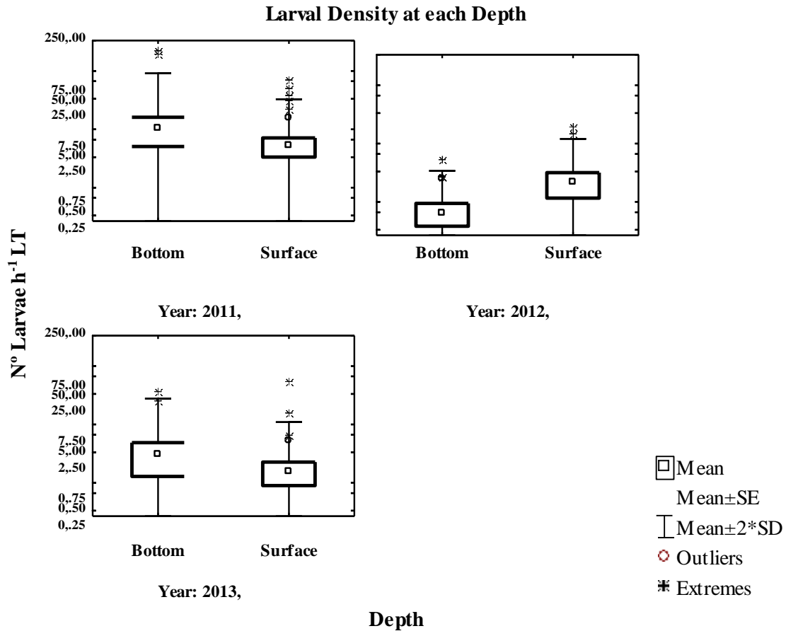
Figure 3.7. Box plots of larval density at each depth strata for light trap samples collected in (A) 2011 (B) 2012 and (C) 2013 plotted on a log scale.
