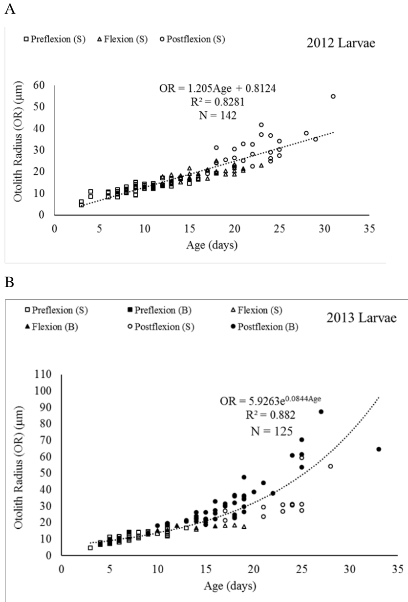
Figure 5.4. Relationship between otolith radius ( OR ; μm) and age (days) for larvae caught in (A) 2012 and (B) 2013. The different developmental stages (preflexion, flexion and postflexion) and the location (S=surface; B=bottom) at which the light trap was set in the water column is differentiated for the larvae.
