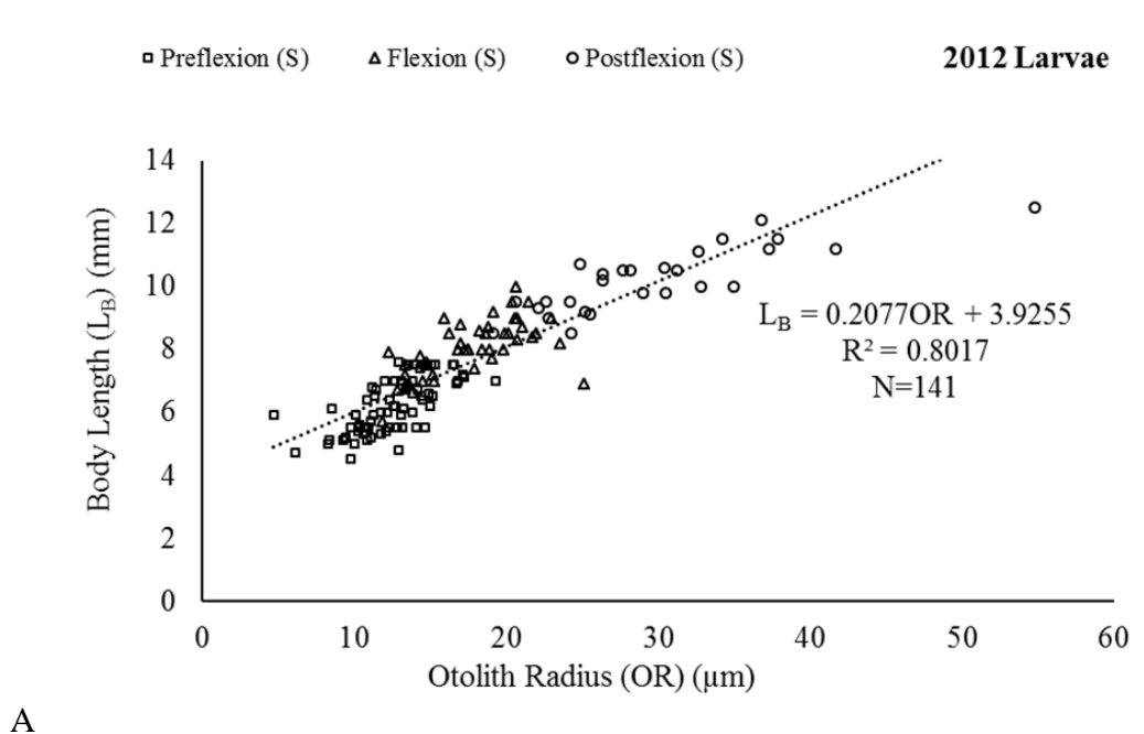
Figure 5.3 (A). Relationship between body length ( L_B ; mm) and otolith radius (OR; \mu\text{m} ) for larvae caught in 2012. The different developmental stages (preflexion, flexion and postflexion) and the location (S=surface; B=bottom) at which the light trap was set in the water column is differentiated for the larvae.
