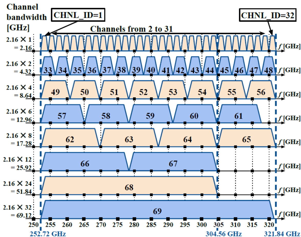
Fig. 7. Channel definition for the IEEE.802.15.3d standard. Taken from [22].
