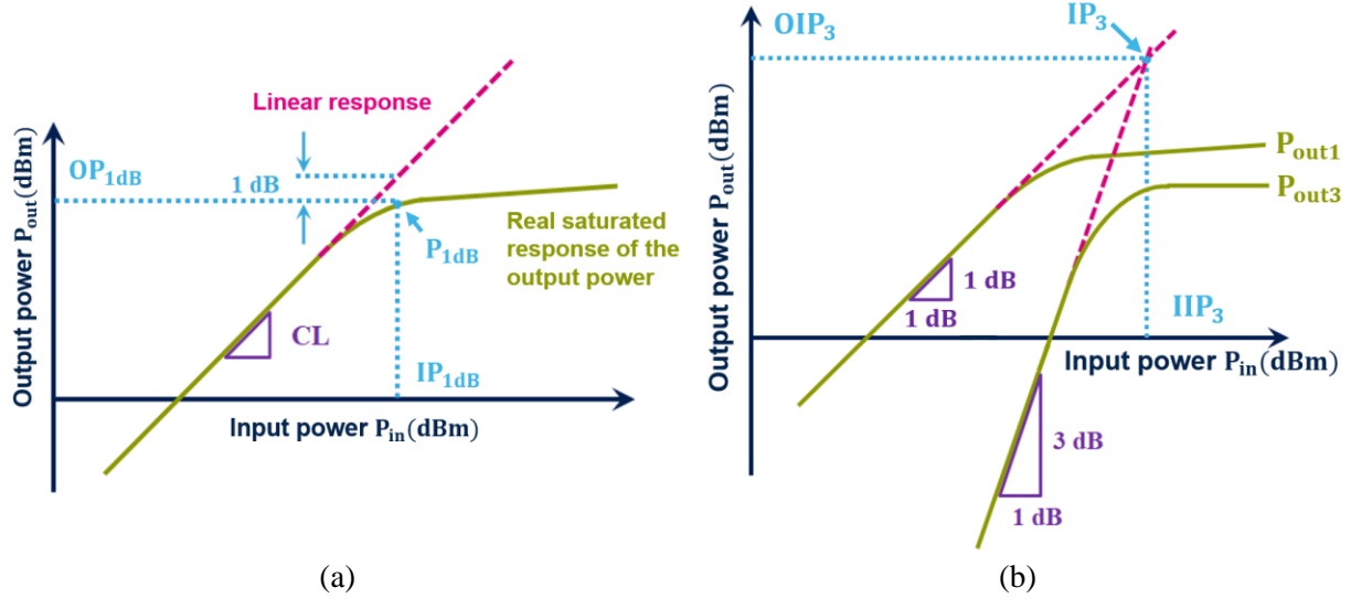
Fig. 26. 1 dB compression point P_{1dB} and determination of third order intermodulation point IP_3 of a mixer. Adapted from [41].
