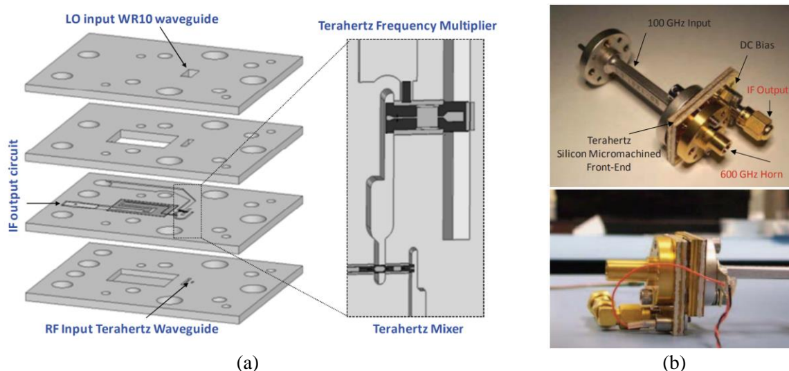
Fig. 58. (a) Silicon micromachined wafers stacked together to form a (b) 600 GHz heterodyne receiver front-end. Taken from [136].
