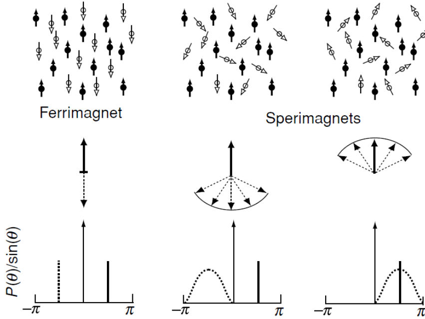
Fig. 3.1: Possible two-sublattice magnetic structures in amorphous binary alloys. At the top Ferrimagnet and sperimagnet atomic spin illustration (RE empty/white spins, TM filled/black spins); at the bottom distribution of local easy axes direction for each sublattice (RE dashed line, TM continuous line). Schematics from [25].
