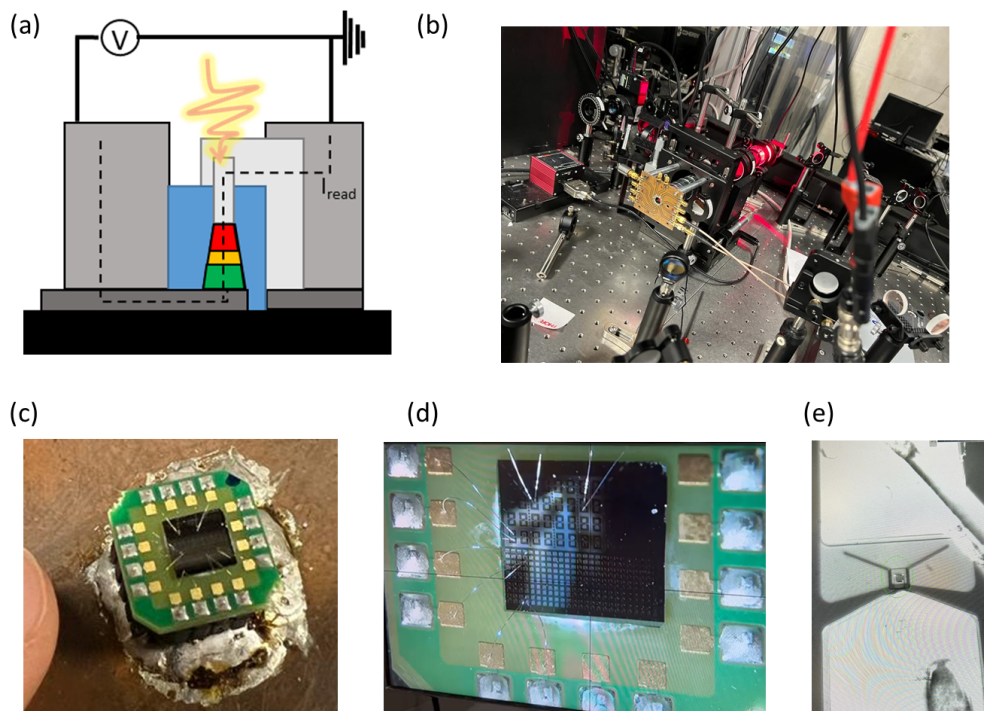
Fig. 5.8: Electrical detected AOS measurement setup. (a) Schematic of the setup; (b) Photo of the sample holder, notice the cables for the electrical measurement; (c-d) Die cut from the wafer with wire-bonding; (e) Microscope image of a device wire-bonded.
