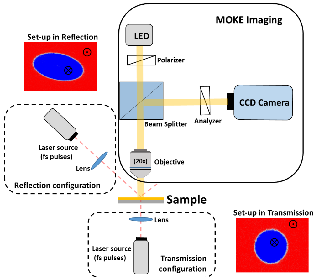
Fig. 2.4: MOKE microscopy setup with single femtosecond laser pulse irradiation.
