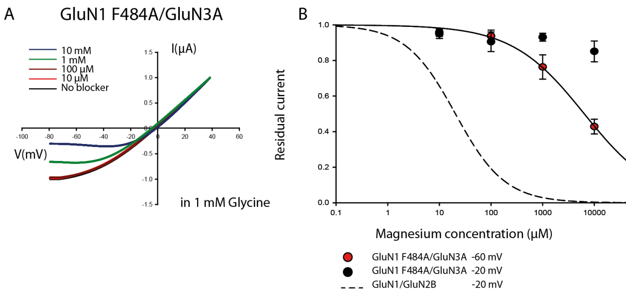
Figure 38 Magnesium sensitivity and IV curve in GluN1 F484A/GluN3A receptors.
