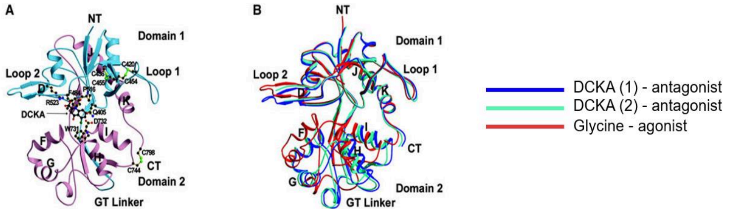
Figure 15 Clamshell conformations change depending on ligand binding.
