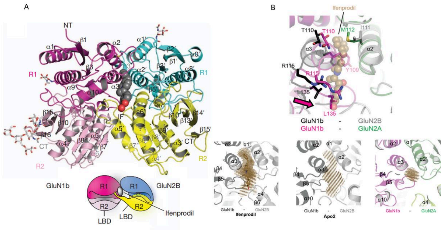
Figure 20 NTD intradimer interface.
