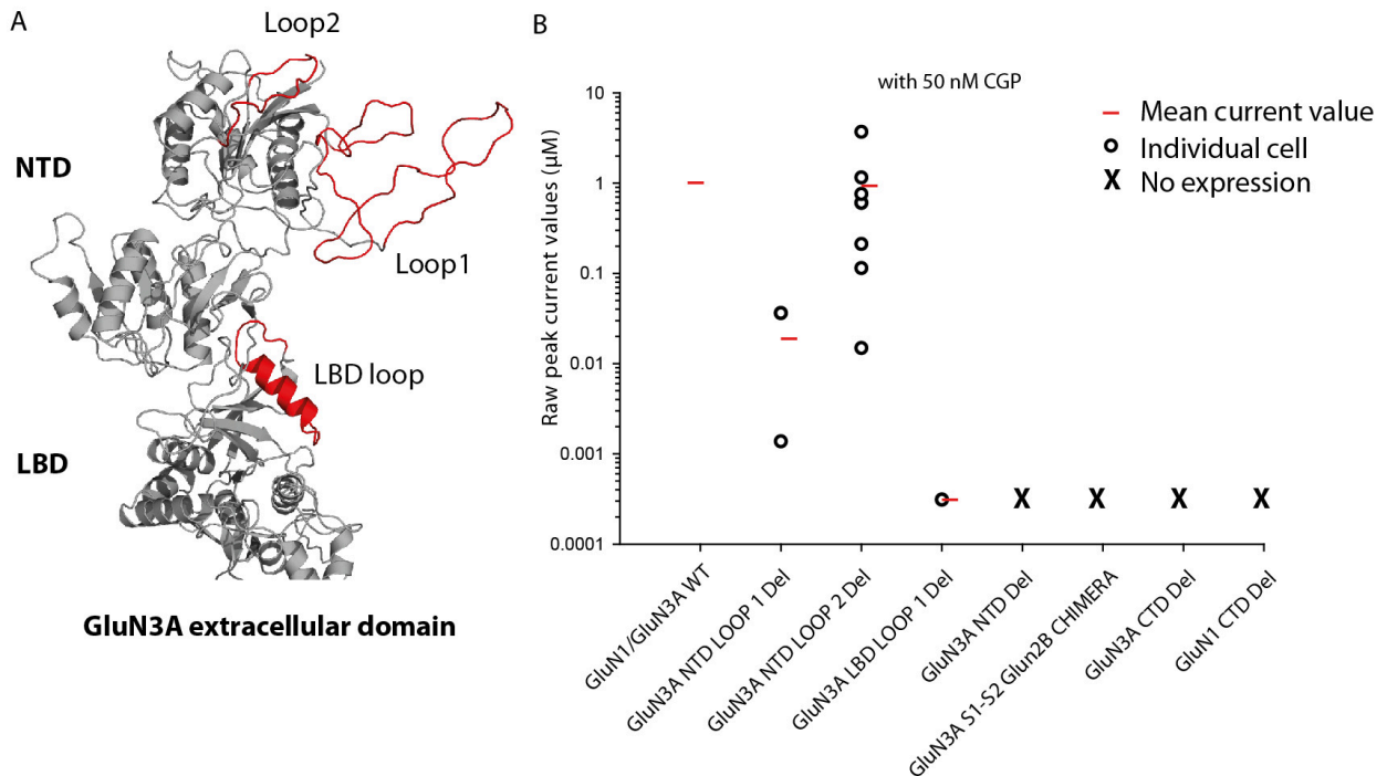
Figure 50 GluN3A deletions and reorganizations.
