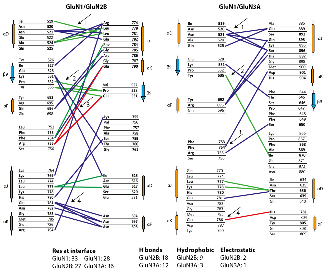
Figure 56 Intradimer Interfaces of GluN1/GluN2B vs GluN1/GluN3A.
