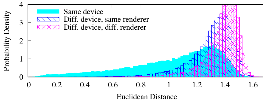
Figure 3.5: Performance of the DRAWNA PART embedding function. A Euclidean distance below 0.65 indicates that the traces are likely to be from the same device.
