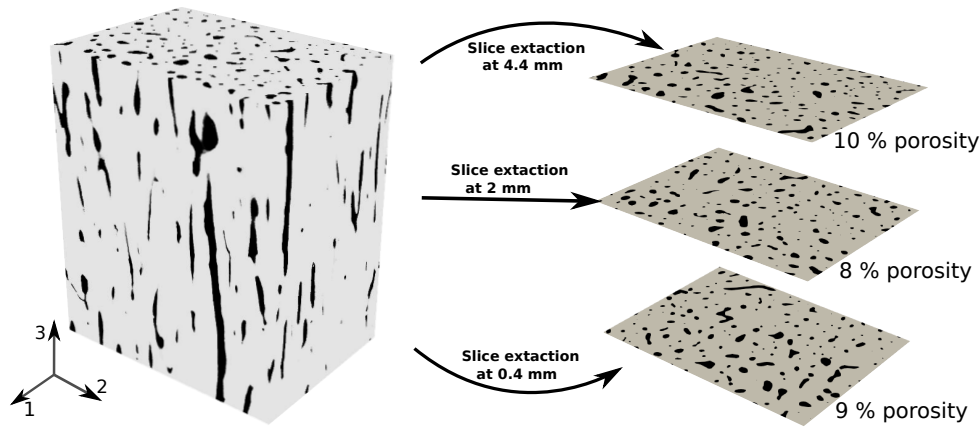
Figure 3.2: Binarized SR- \mu CT image of a cortical bone specimen of nominal dimensions 3 \times 4 \times 5 \text{ mm}^3 (original voxel size 6.5 \mu\text{m} ). Black: vascular pores; light gray: mineralized matrix. Axis 1 corresponds to radial direction, axis 2 to the circumferential direction and axis 3 to the axial direction or diaphysis axis. For illustration, 3 slices extracted from the 3D volume, as used for 2D numerical simulations, are shown. 2D porosity values are given for each slice, illustrating the variable porosity in a 3D volume
