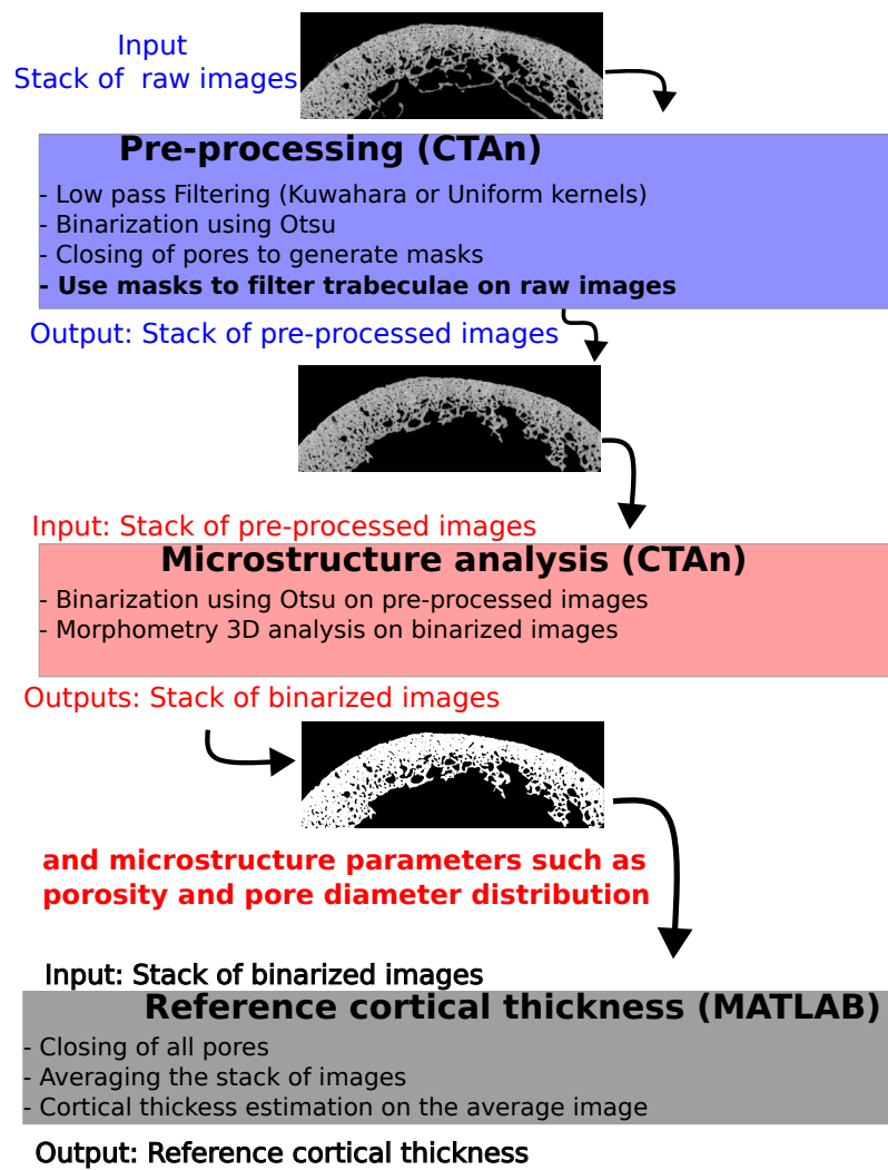
Figure 4.8: Summary of all the steps involved in the microstructure analysis and the determination of the reference cortical thickness.
