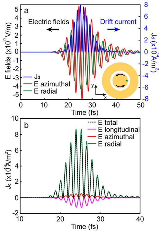
Figure 2.4 : Temporal response of drift currents. (a) Temporal evolution of the drift currents (blue curve), superimposed on the temporal evolution of the radially (green curve) and azimuthally (red curve) polarized electric fields, inside the metal core of the plasmonic nanoantenna, symbolized by the green star in the inset drawing. (b) Contribution of the different components, longitudinal (along z), azimuthal and radial, of the electric optical field in generating drift currents.
