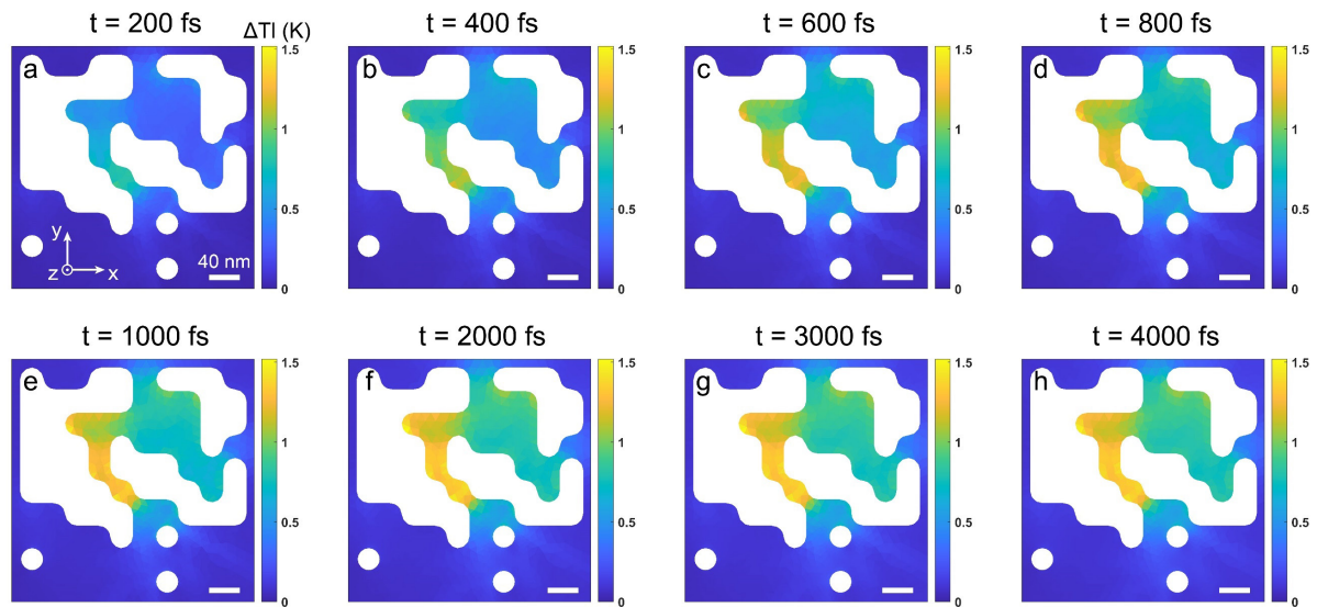
Figure 6.4 : Spatial distribution of lattice temperature generation in an XY plane at the Z center of the optimized nanostructure for different characteristic times after the optical pulse, a) 200 fs, b) 400 fs, c) 600 fs, d) 800 fs, e) 1000 fs, f) 2000 fs, g) 3000 fs, h) 4000 fs.
