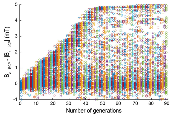
Figure 4.3 : Evolutionary process. Evolution during the different generations of the optimization function consisting in maximizing the difference \mathbf{B}_{z-RCP} - \text{abs}(\mathbf{B}_{z-LCP}) , with \mathbf{B}_{z-RCP} and \mathbf{B}_{z-LCP} the \mathbf{B} -fields created by a right or left circular polarization, respectively. Each generation consists of 200 structures. The optimized structure appears after 76 generations.
