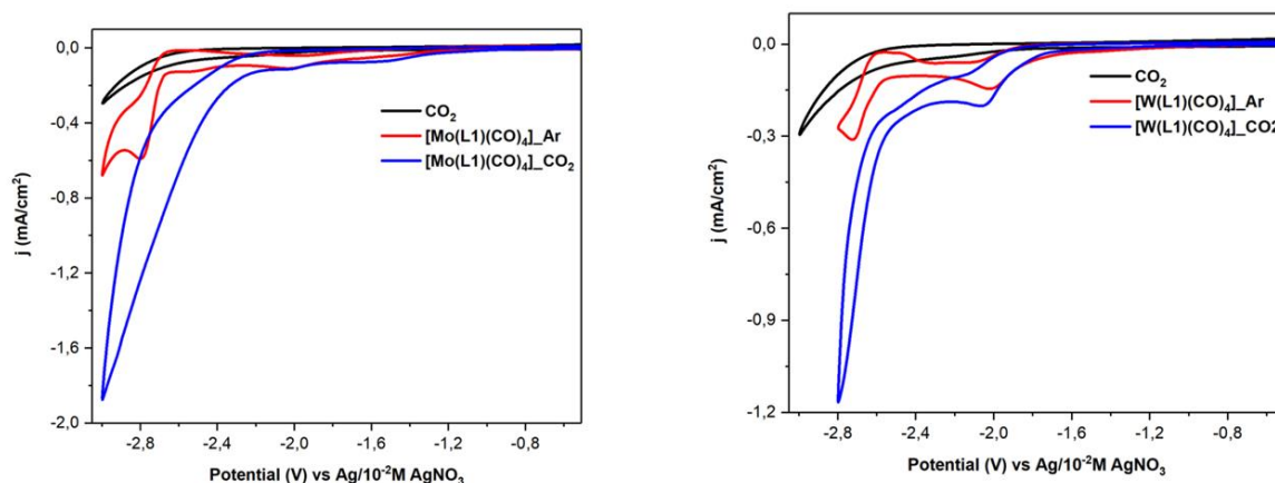
Figure III. 6 Cathodic CV scans of a 1mM [M(L1)(CO)_4] complex under CO 2 saturated conditions on GCE in CH_3CN/0,1M TBAPF 6 at \nu = 0.05 Vs -1 .
