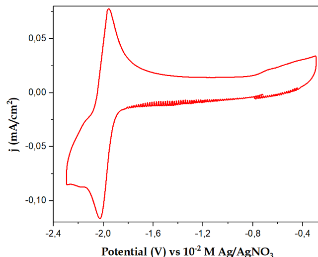
Figure IV. 23 Cathodic CV scan of a 1mM [Cu(bph)(POP)] + complex under argon saturated conditions on GCE in DMF/0,1M TBAPF 6 at \nu = 0.1 \text{ Vs}^{-1} .
