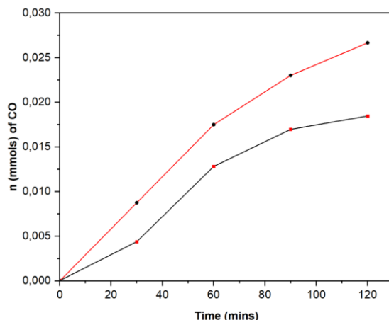
Figure IV. 18 Evolution of the number of moles of CO produced in two different days during electrolysis of 1mM [\text{Cr}(\text{qpy})(\text{Cl})_2]^+ complex at -1.85\text{V} \text{Ag}/10^{-2}\text{M} \text{AgNO}_3 under \text{CO}_2 saturated conditions with 1.5M of PhOH on a carbon foam in DMF/0,1M \text{TBAPF}_6 .
