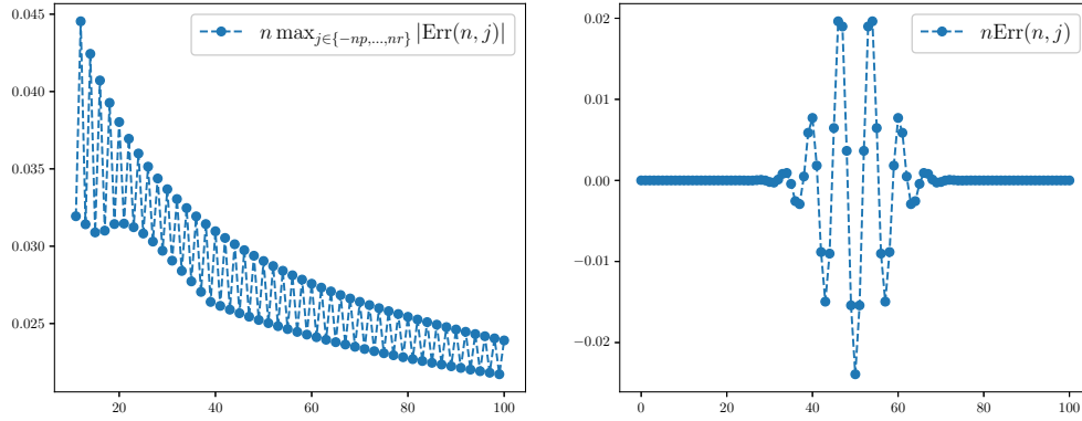
Figure 2.8 – For these figures, we chose \lambda a = 1/2 . On the left : A representation of n \max_{j \in \{-nr, \dots, nr\}} |\text{Err}(n, j)| depending on n . As expected, the function seems to be bounded. On the right : We fixed n = 100 and represented j \in \mathbb{Z} \mapsto n\text{Err}(n, j) . We observe the exponential decay in j . Also, we can see a particular shape of curve that arises that would correspond to the next term in the asymptotic expansion of \mathcal{G}_j^n .
