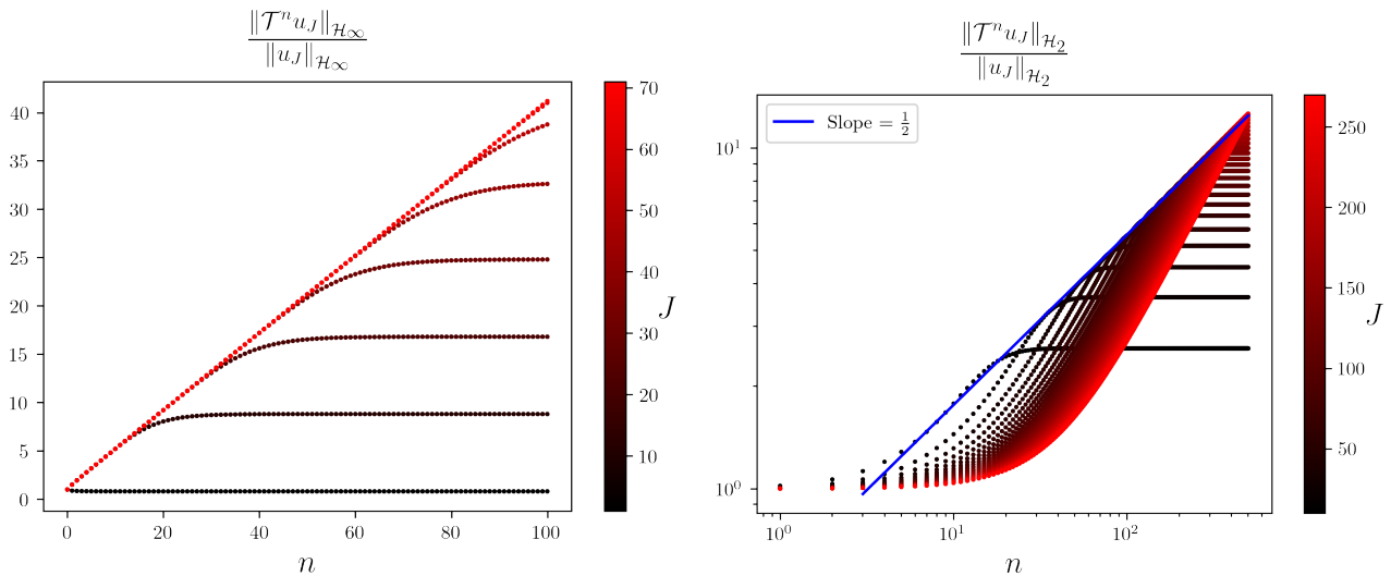
Figure 3.5 – We consider the modified Lax-Friedrichs scheme (3.2.1). On the left side: For several choices of integers J , we compute the ratio between \|\mathcal{T}^n u_J\|_{\mathcal{H}_\infty} and \|u_J\|_{\mathcal{H}_\infty} depending on n , where the sequence u_J is defined by (3.2.5). For n fixed, this gives a lower bound for \|\mathcal{T}^n\|_{\mathcal{L}(\mathcal{H}_\infty)} . The figure supports the fact that \|\mathcal{T}^n\|_{\mathcal{L}(\mathcal{H}_\infty)} grows at a linear rate with regards to n . On the right side: For several choices of integers J , we compute the ratio between \|\mathcal{T}^n u_J\|_{\mathcal{H}_2} and \|u_J\|_{\mathcal{H}_2} depending on n , where the sequence u_J is defined by (3.2.5). For n fixed, this gives a lower bound for \|\mathcal{T}^n\|_{\mathcal{L}(\mathcal{H}_2)} . The representation in the logarithmic scale supports the fact that \|\mathcal{T}^n\|_{\mathcal{L}(\mathcal{H}_2)} grows at a rate \sqrt{n} .
