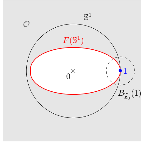
Figure 3.1 – An example of curve F(\mathbb{S}^1) . Hypothesis 3.1 implies that the curve F(\mathbb{S}^1) (in red) is inside the closed disk \mathbb{D} and touches the boundary \mathbb{S}^1 only at 1. In gray, we have \mathcal{O} the unbounded connected component of \mathbb{C} \setminus F(\mathbb{S}^1) . In dashed, we find the ball B_{\tilde{\varepsilon}_0}(1) where we have a more precise spectral decomposition (3.1.14) associated with the matrix \mathbb{M}(z) defined by (3.1.12).
