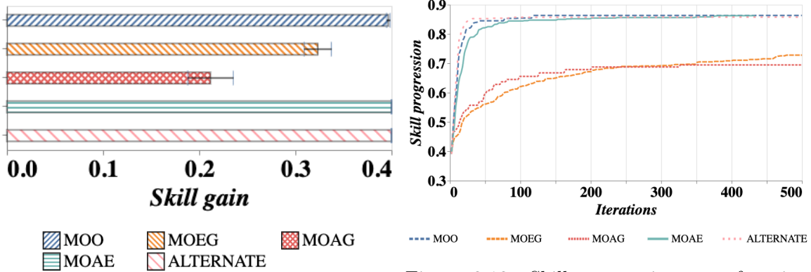
Figure 3.12: Average skill gain with variable initial skills for learners. Figure 3.13: Skill progression as a function of # iterations with variable initial skills for learners.
