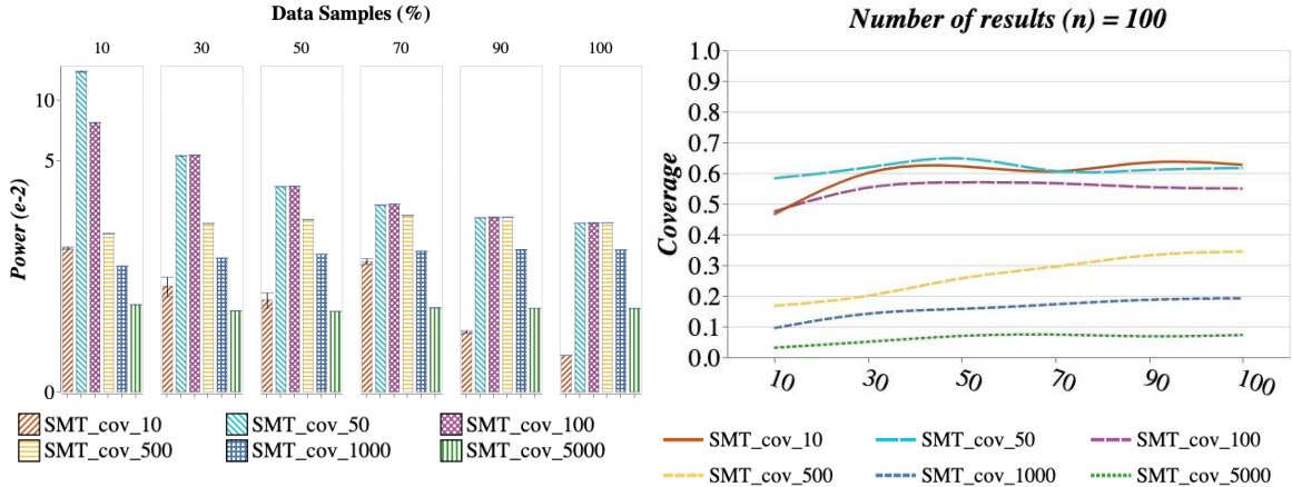
Figure 4.3: Impact of coverage optimization on Power with cov_{min} = 0.5 and number of results n = 100 for different percentages of data samples.
