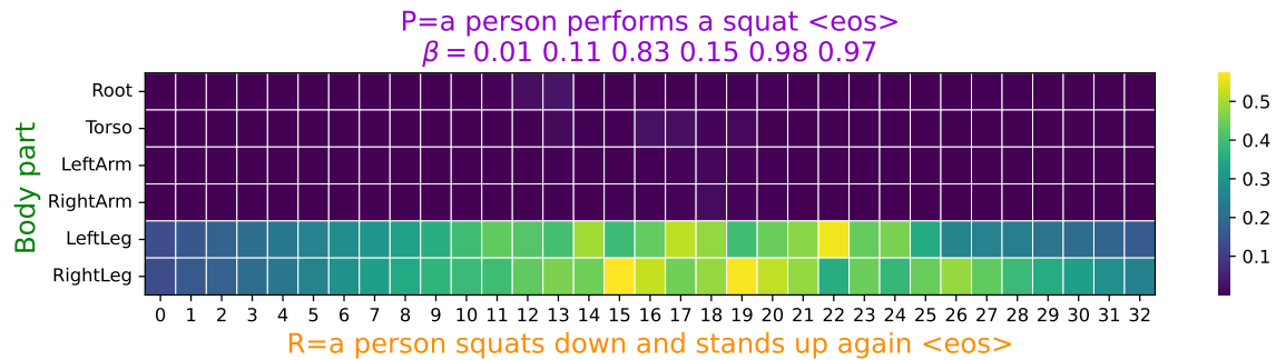
(c) Squat (action range [10,28]).
