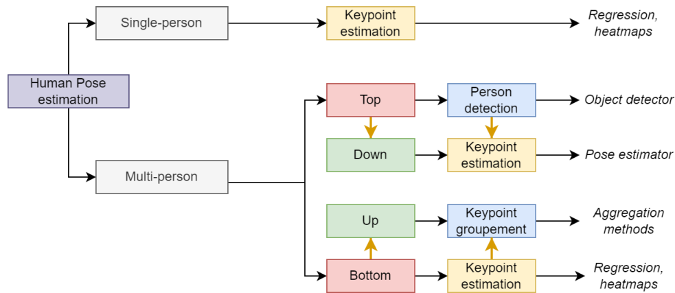
FIGURE 2.3: Overview: Top-down vs. bottom-up approach for HPE.
