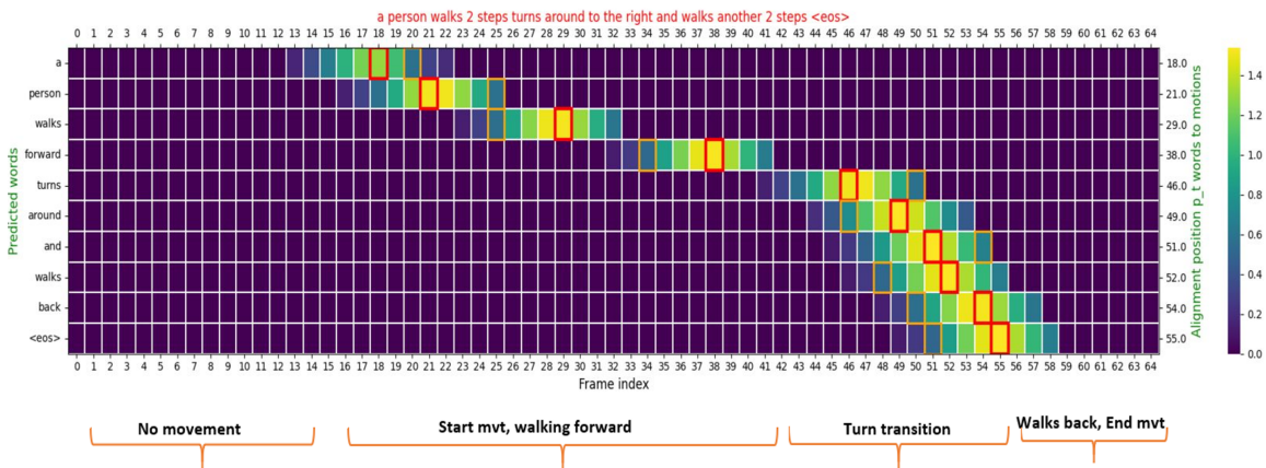
FIGURE 4.33: walk forward: \llbracket 15, 38 \rrbracket , turn at frame 40, walk backward: \llbracket 42, 53 \rrbracket .
