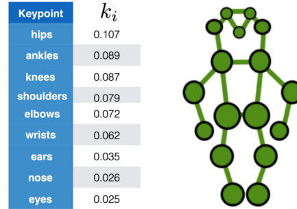
FIGURE 2.20: The k_i constants calculated for the skeleton format of the COCO dataset.
