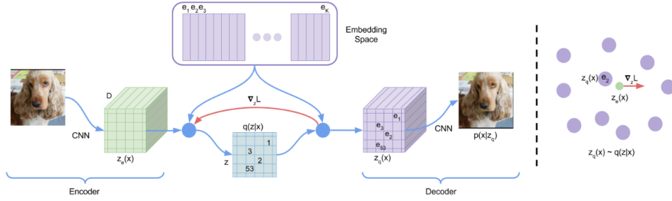
FIGURE 4.1: The VQ-VAE architecture (van den Oord et al., 2017).
