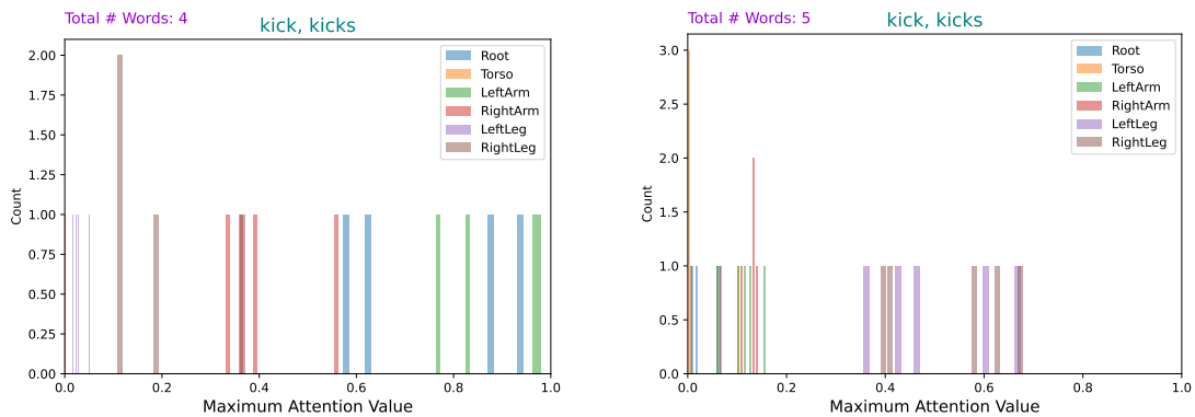
(a) Without spatial supervision, model incorrectly focuses on arms/root for the word "kicks".
