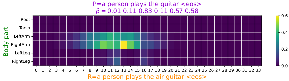
(a) Play (action range [10,20]).
