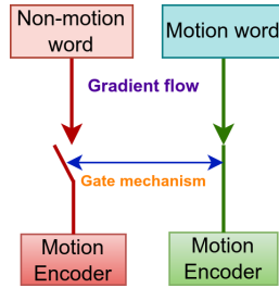
FIGURE 6.11: Illustration of our gating mechanism during training. The motion encoder is prevented from receiving important gradient updates for non-motion words.
