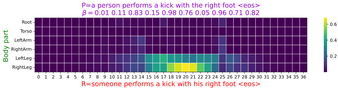
(b) KIT-(2,3), word kick
