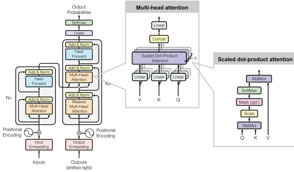
FIGURE 4.12: Transformer model compounds (Vaswani et al., 2017).
