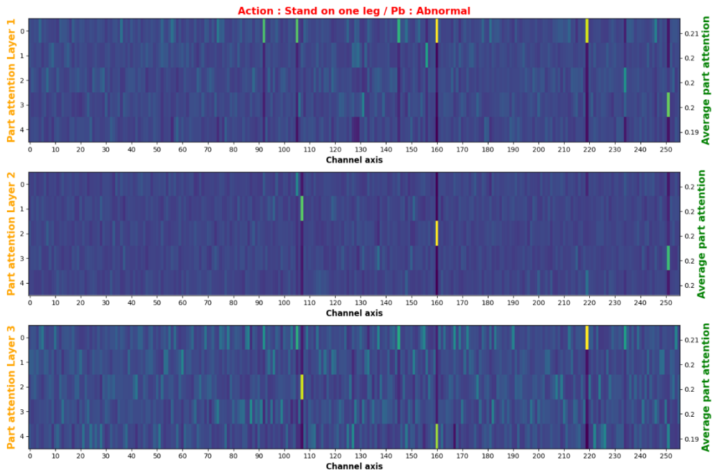
(b) Last 3 layers of Part attention with channel dimension of 256.
