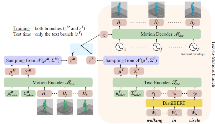
FIGURE 4.7: Motion generation with Transformer-based VAE (Petrovich et al., 2022).
