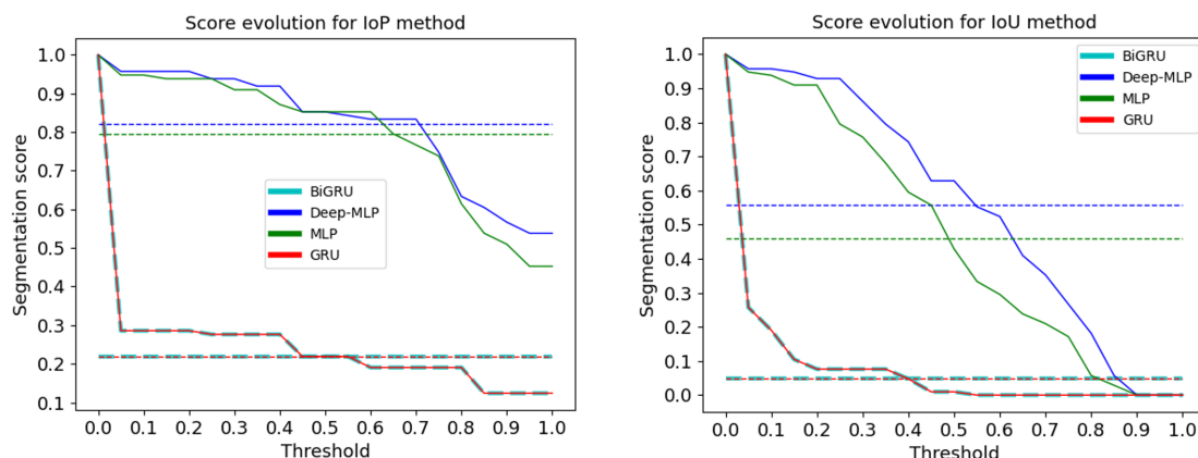
FIGURE 5.5: Comparison of IoP and IoU scoring methods. The legend specifies the encoder types, and the dashed lines represent the average segmentation scores (Radouane et al., 2023a).
