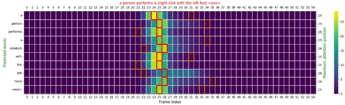
FIGURE 4.20: BiGRU-cartesian[Soft.att] : Kick in the range \llbracket 20, 35 \rrbracket .
