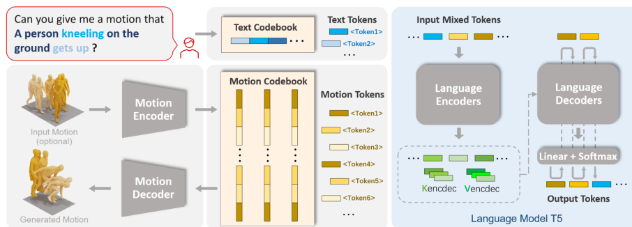
FIGURE 4.11: MotionGPT: Overview of framework design for multitask learning (Jiang et al., 2024).
