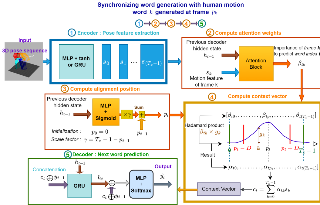
FIGURE 4.15: The five steps illustrating the motion to language generation (3D animation for synchronous generation of text with motion can be found in the Code).
