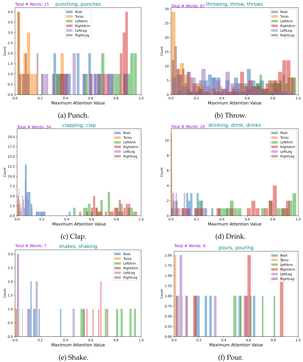
FIGURE 6.15: Histograms generated on the HML3D with the config (0,3).
