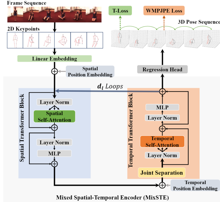
FIGURE 2.13: MixSTE architecture design (Zhang et al., 2022).
