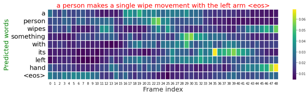
FIGURE 4.31: Transformer [H1L1] cross attention visualization ( Wiping ).
