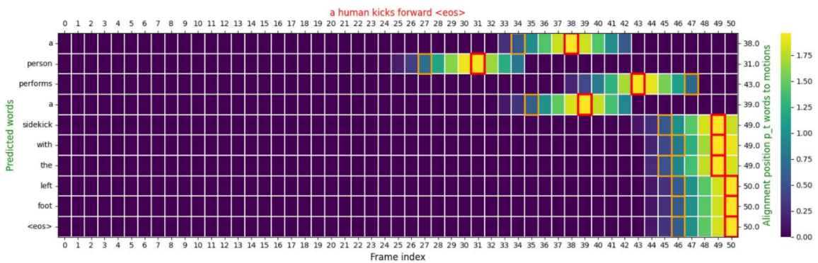
FIGURE 4.23: BiGRU[Local.att] kick action in the range [[10, 28]
