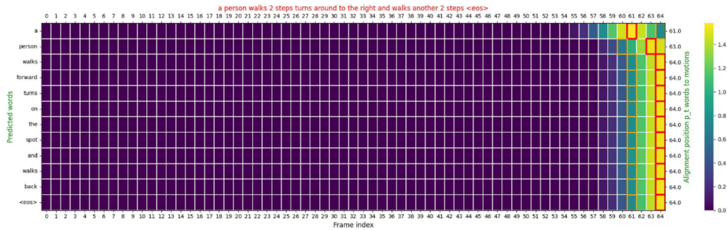
FIGURE 4.24: BiGRU[Local.att]: Walk forward [[15, 38]] , Turn around [[39, 48]] and Walk backward [[49, 53]]
