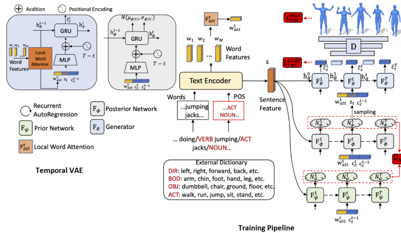
FIGURE 4.6: Motion generation based on GRU and motion snippet code (Guo et al., 2022a).
