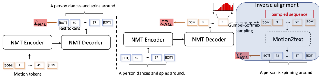
FIGURE 4.8: Motion generation with motion tokens as an NMT task (Guo et al., 2022a).
