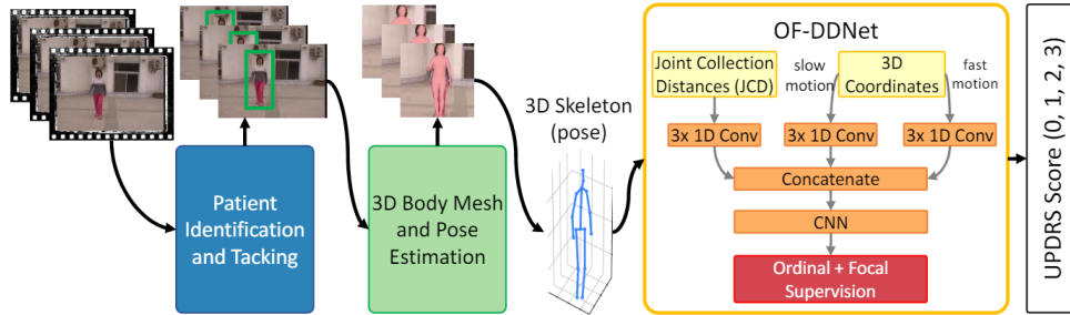
FIGURE 3.1: Architecture OF-DDNET
