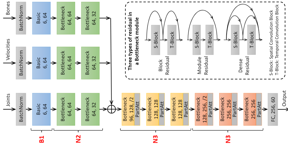
FIGURE 3.9: Part Attention Residual GCN architecture (Song et al., 2020).
