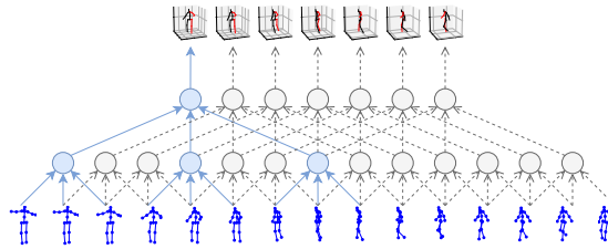
(b) Dilated convolutions for 2D-3D pose regression.
