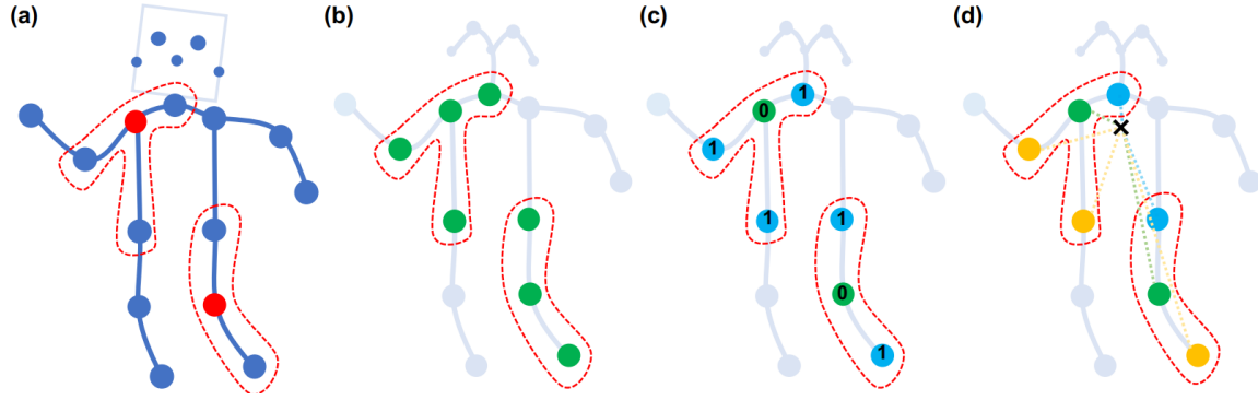
FIGURE 3.7: Human skeleton partitioning configurations Yan et al. (2018).
