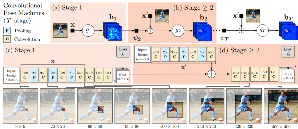
FIGURE 2.7: Convolutional pose Machines (Wei et al., 2016).
