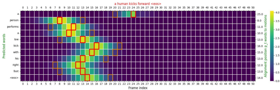
FIGURE 4.21: BiGRU[Local.att Mask False]: Kick action in the range \llbracket 10, 28 \rrbracket
