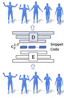
FIGURE 4.4: The auto-encoder architecture ( E - D ) comprises two-layer convolutions with a filter size of 4 and a stride of 2 (Guo et al., 2022a).
