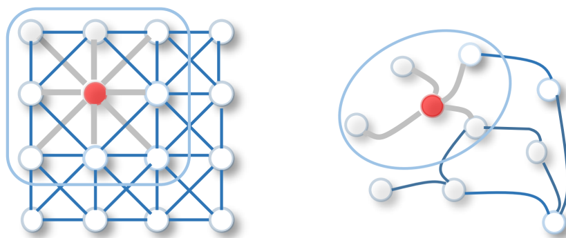
FIGURE 3.5: Comparison of convolution on an image and convolution on a graph (Wu et al., 2019).
