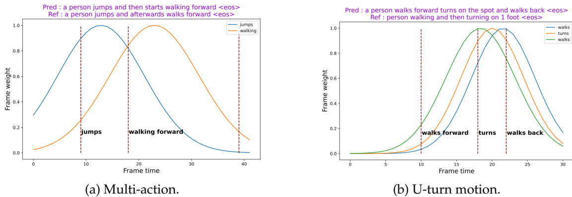
FIGURE 6.10: Temporal gaussian window displayed for different motion words given a prediction on KIT-ML.
