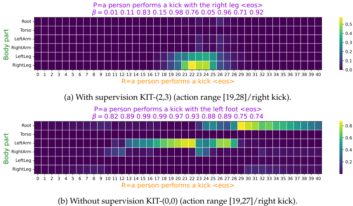
FIGURE 6.12: Comparison between the case of guided attention and no supervision.
