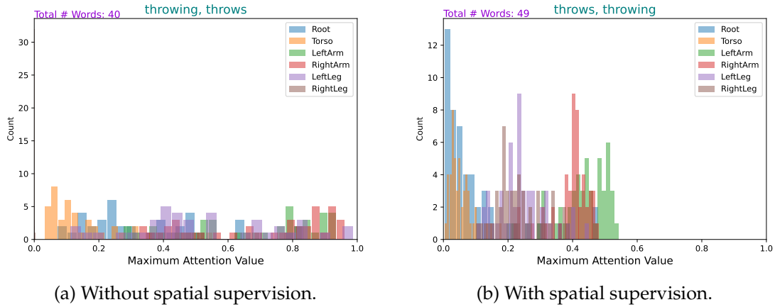
FIGURE 6.9: Effect of spatial supervision on Human-ML3D.
