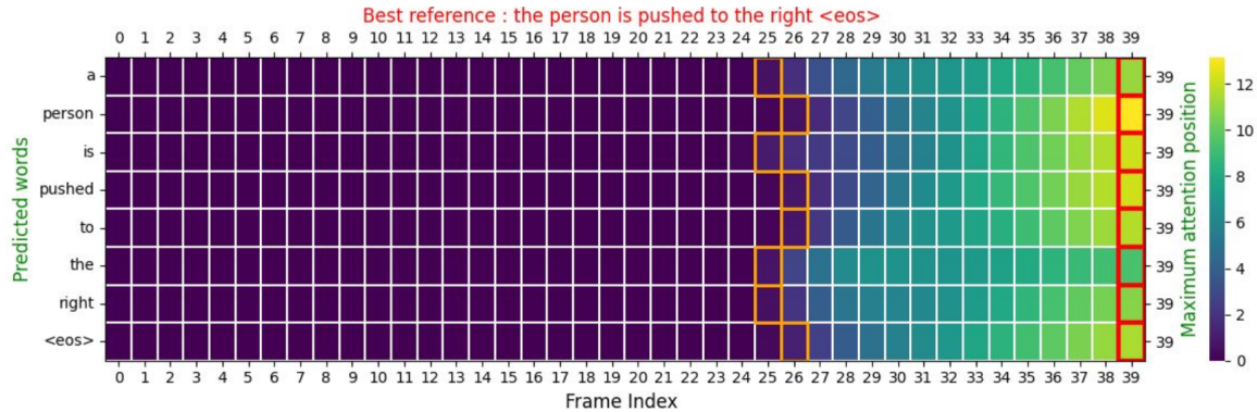
FIGURE 4.18: GRU-cartesian[Soft.att]: Pushing action in the range \llbracket 11, 20 \rrbracket .
