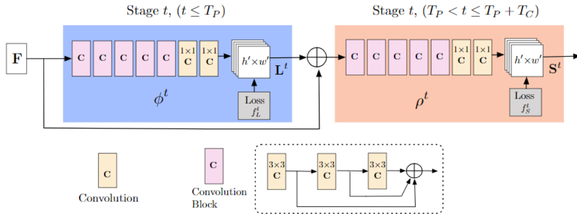
FIGURE 2.9: Open pose CNN-based operations.
