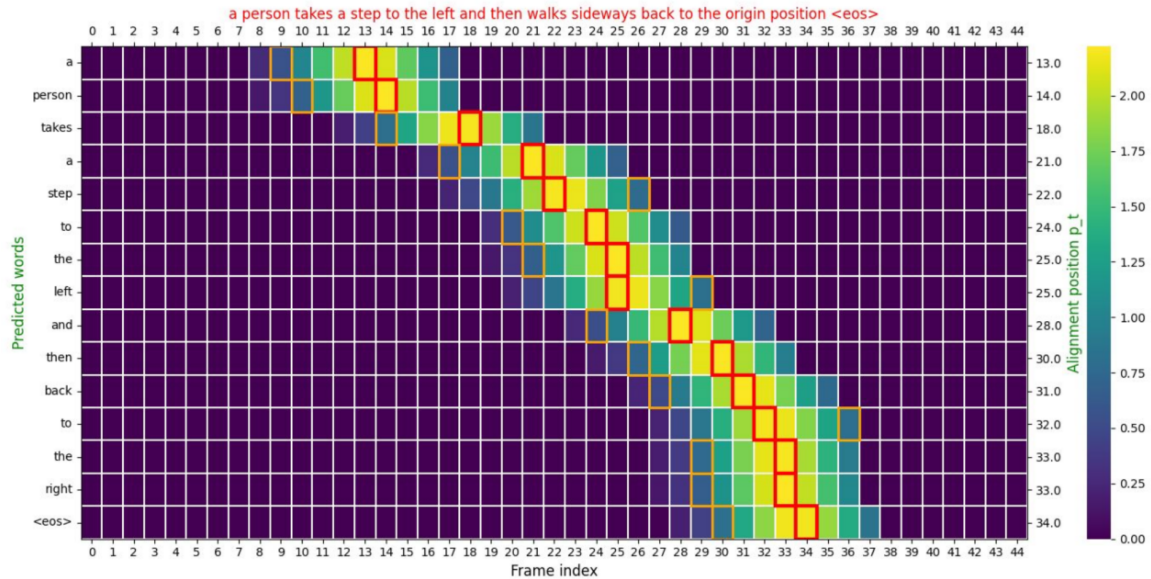
FIGURE 4.30: DeepMLP[Local.rec.att] D = 5 : Move to the left in the range [[8, 23]] , move to the right in the range [[24, 35]]
