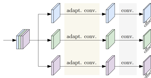
FIGURE 2.10: Disentangled keypoint regression (Geng et al., 2021).
