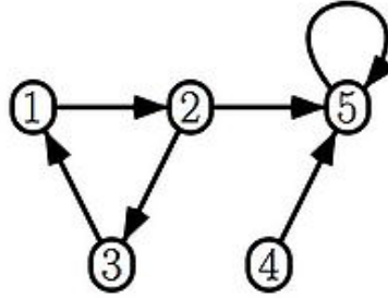
FIGURE 3.4: Example of a directed graph.
