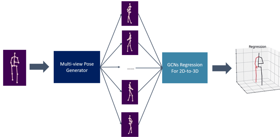
FIGURE 2.12: Multi-view generation architecture (MvPG) and 3D reconstruction (GCNs) (Sun et al., 2020).
