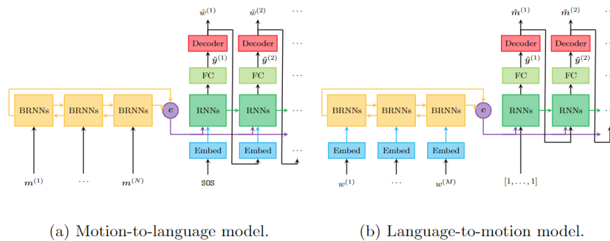
FIGURE 4.5: The bidirectional mapping model proposed by (Plappert et al., 2018).
