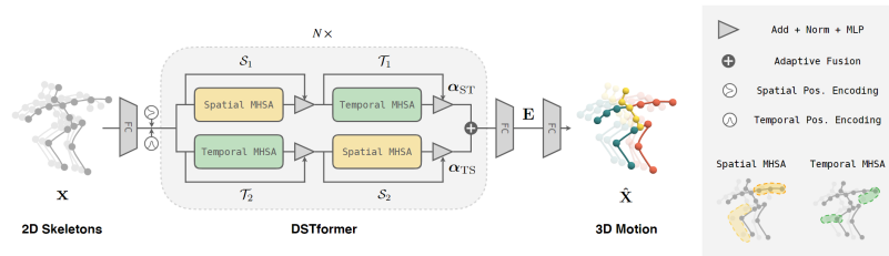
(b) Transformer-based model architecture.
