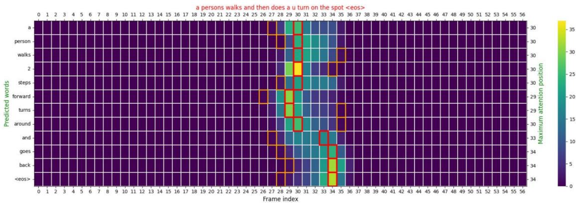
FIGURE 4.19: BiGRU-cartesian[Soft.att]: Walk forward in the range \llbracket 0, 28 \rrbracket , Turn around \llbracket 29, 35 \rrbracket and Walk backward \llbracket 36, 56 \rrbracket .
