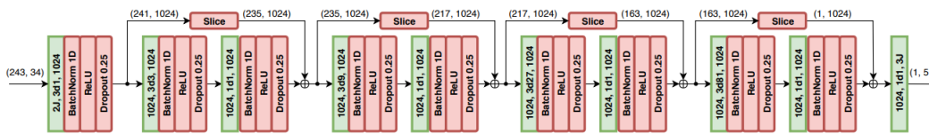
(a) Videopose3D architecture.
