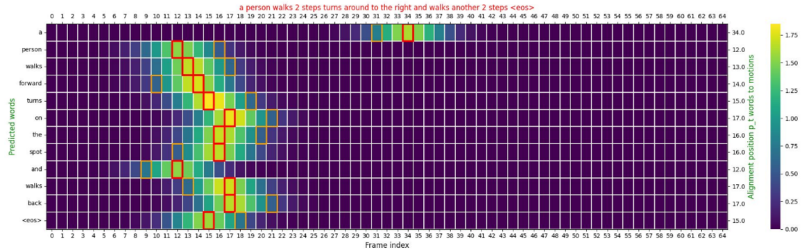
FIGURE 4.22: BiGRU[Local.att Mask False]: Walk forward [[15, 38] , Turn around [[39, 48] and Walk backward [[49, 53]
