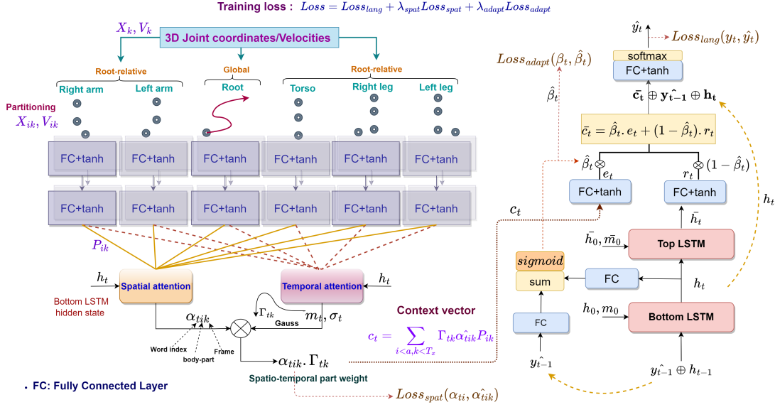
FIGURE 6.3: Our architecture design with an MLP-based encoder, and Two LSTM-based decoders (Radouane et al., 2023b).
