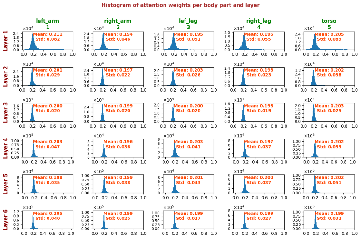
FIGURE 3.15: Attention distribution per part and layer across all validation samples.
