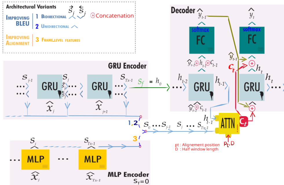
FIGURE 4.16: Experimented architectures, GRU, Bi-GRU and MLP-GRU (The word embedding layer is not represented).
