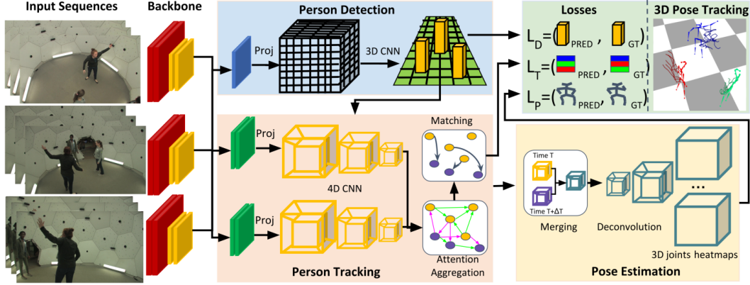
FIGURE 2.19: TESSE-TRACK : Multitask learning for multi-person pose estimation and tracking.
