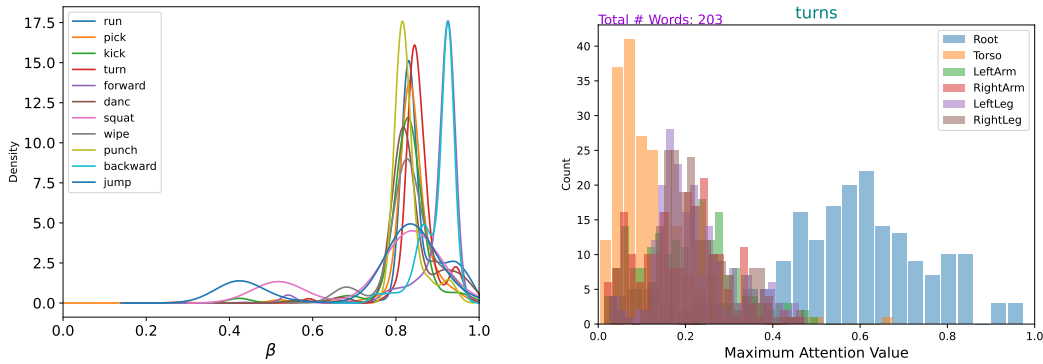
(a) With gate supervision, motion information is correctly used frequently for motion-words generation. (b) Attention is frequently focused on relevant parts: e.g. on Root (global trajectory) for word "turns".
