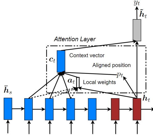
FIGURE 4.13: Schematic description of the process of encoding and decoding, which involve the computation of alignment position p_t (Luong et al., 2015).
