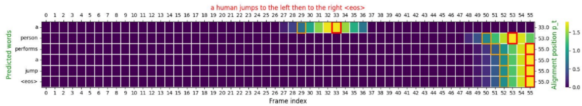
FIGURE 4.26: GRU[Loc.rec.att]: Jump to the left [[0, 31]] , Jump to the right [[32, 54]]
