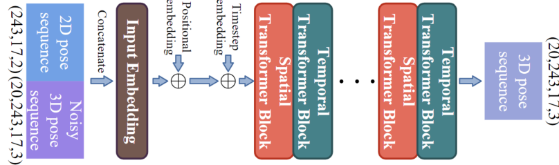
(b) Denoiser architecture where 20, 243, 17 are the number of hypotheses H , frames N , and human joints J in each frame, respectively.
