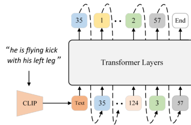
FIGURE 4.9: T2M-GPT architecture for text-to-motion generation (Zhang et al., 2023).
