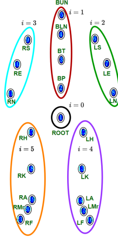
FIGURE 6.4: Partitioning of KIT skeleton of 21 joints into 6 body parts (22 joints for Human-ML3D) (Radouane et al., 2023b).
