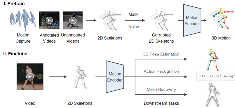
(a) Framework overview as two processes.
