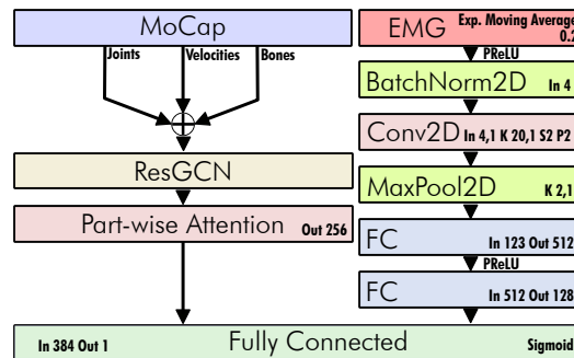
FIGURE 3.11: Architecture of the multimodal PA-ResGCN-N51 + EMG CNN system (Radouane et al., 2021).
