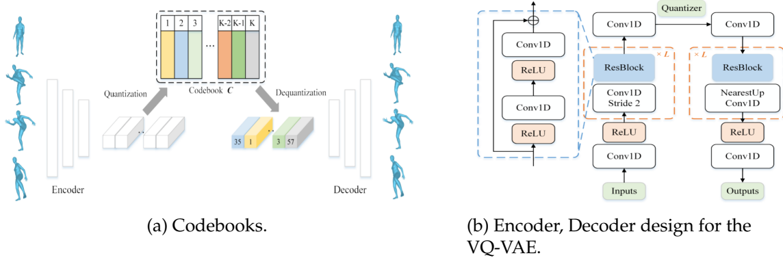
FIGURE 4.3: Codebooks learning details (Zhang et al., 2023).
