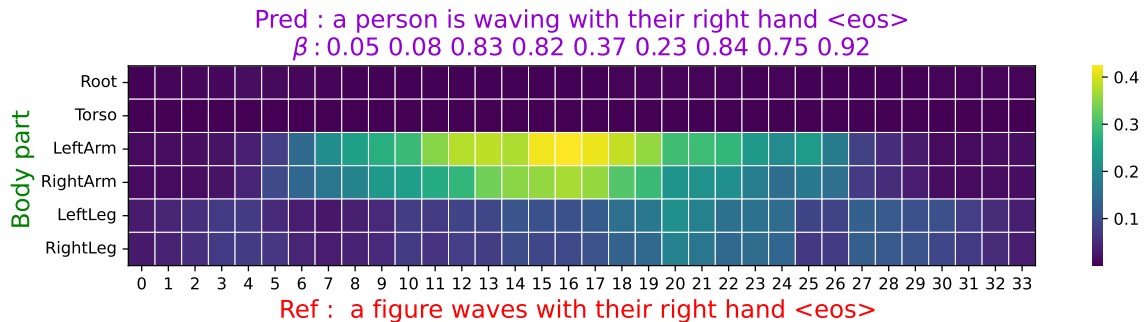
(a) HML3D-(2,3), word waving
