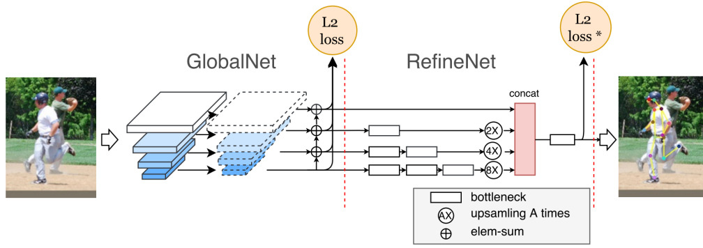
(a) Architecture of the CPN (Cascaded Pyramid Network).
