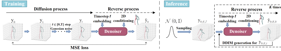
(a) Overview of HPE based on diffusion process.
