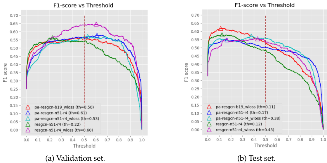
FIGURE 3.13: F1 score as function of threshold. Optimal thresholds are denoted as th in the legend.
