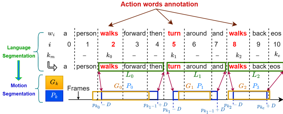
FIGURE 5.4: The language and segmentation process applied on an example of predicted words w_i with given action words and frame annotations G_k . The inferred motion segment is P_k and the language segment is L_k . The index k_e always refers to the end token (Radouane et al., 2023a).
