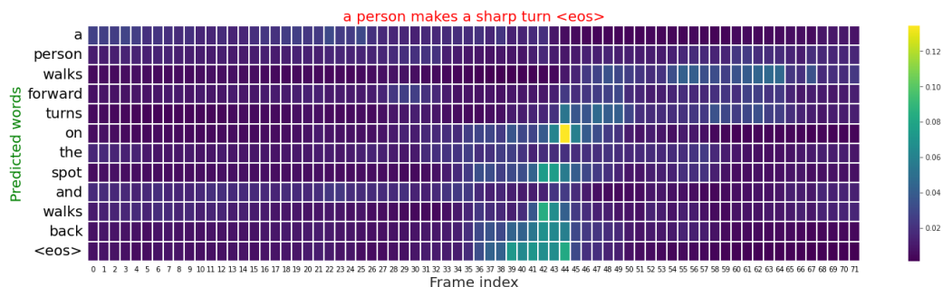
FIGURE 4.32: Transformer [H1L1] cross-attention visualization ( U-turn ).
