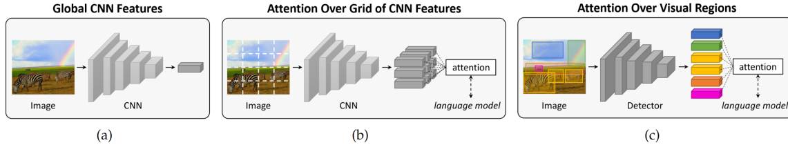
FIGURE 6.1: Different methods for image feature extraction (Stefanini et al., 2023).
