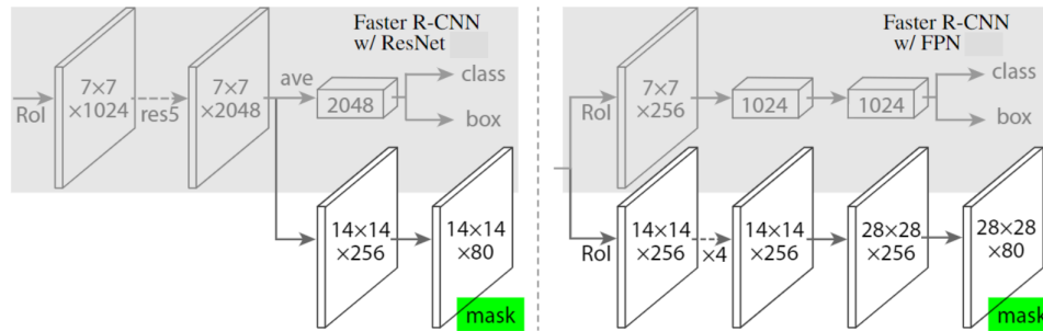
FIGURE 2.5: The head of the MASK-RCNN architecture (He et al., 2017).
