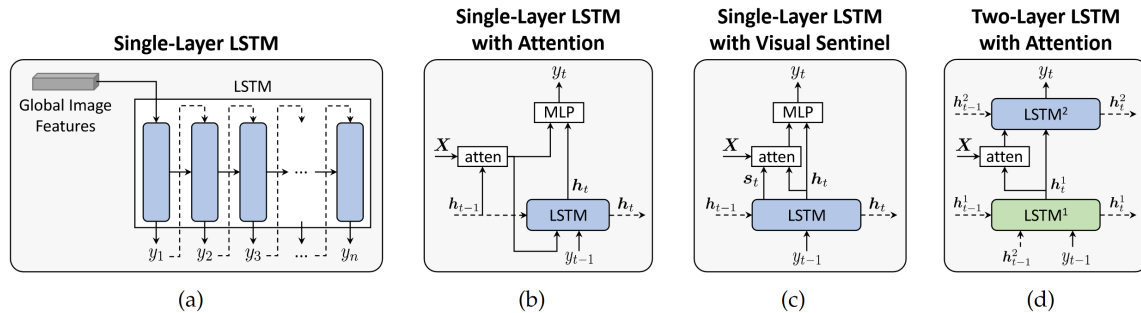
FIGURE 6.2: LSTM-based decoder. (a) No attention, (b)-(c)-(d) different methods for attention score computation (Stefanini et al., 2023).
