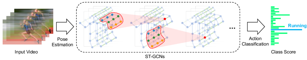
FIGURE 3.6: ST-GCN (Yan et al., 2018)
