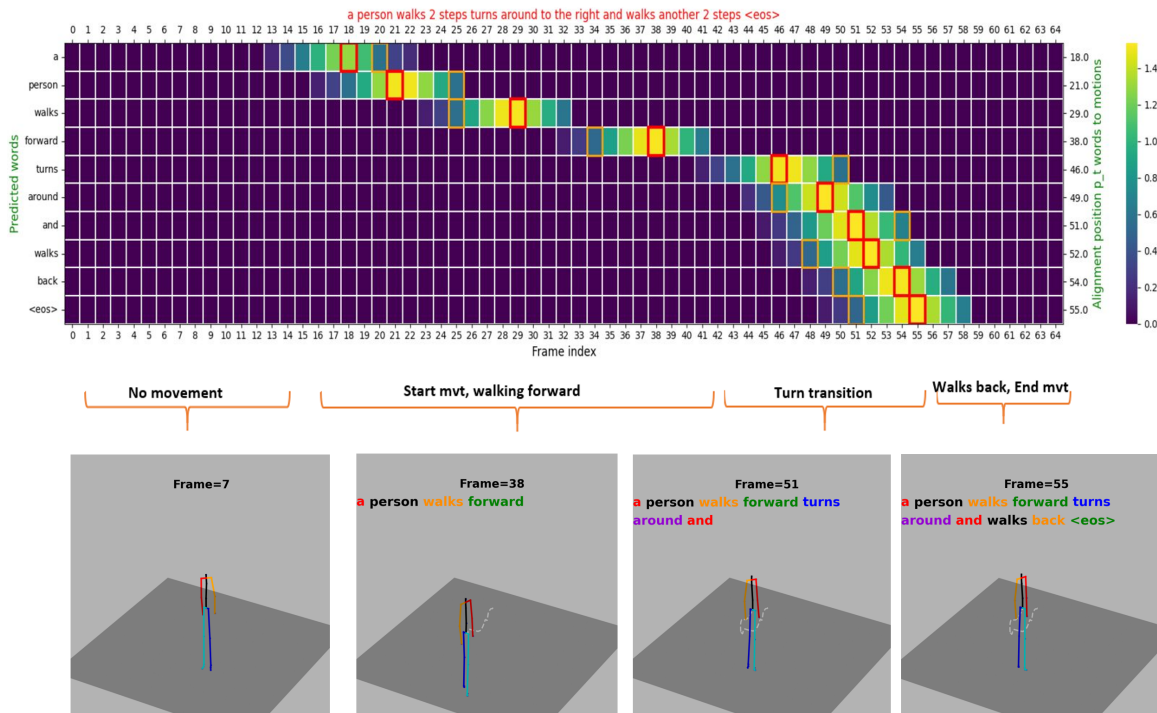
FIGURE 5.6: MLP-GRU [Local.rec.att Mask True D = 5 ]: walk forward in the range \llbracket 15, 38 \rrbracket , turn at frame 40, walk backward in \llbracket 42, 53 \rrbracket
