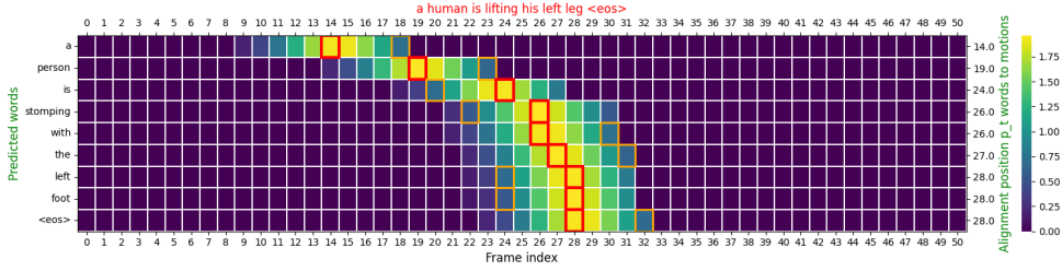
FIGURE 5.7: Truncated Gaussian MLP-GRU with D = 5 , Stomping action at \llbracket 22, 30 \rrbracket .
