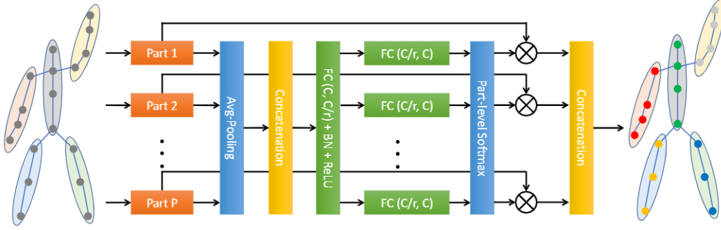
FIGURE 3.10: Attention weights computation (Song et al., 2020).
