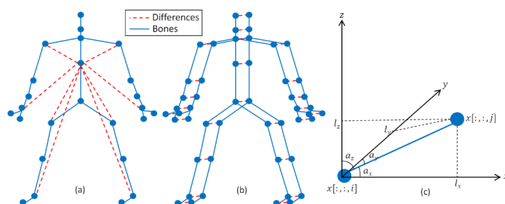
FIGURE 3.3: The demonstration of input data: (a) is the relative positions, (b) is the motion velocities, and (c) demonstrates the 3D lengths and the 3D angles of a bone. (Song et al., 2020)
