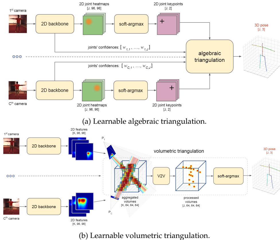
FIGURE 2.16: Two triangulation-based methods for 3D multi-view pose estimation.
