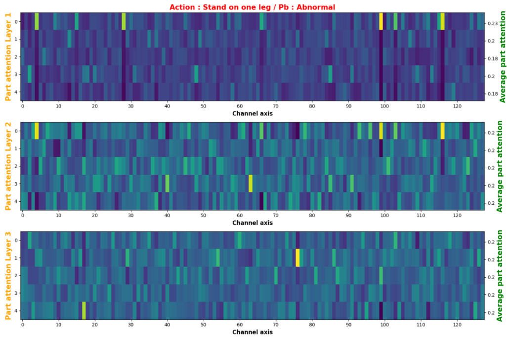
(a) First 3 layers of Part attention with channel dimension of 128.
