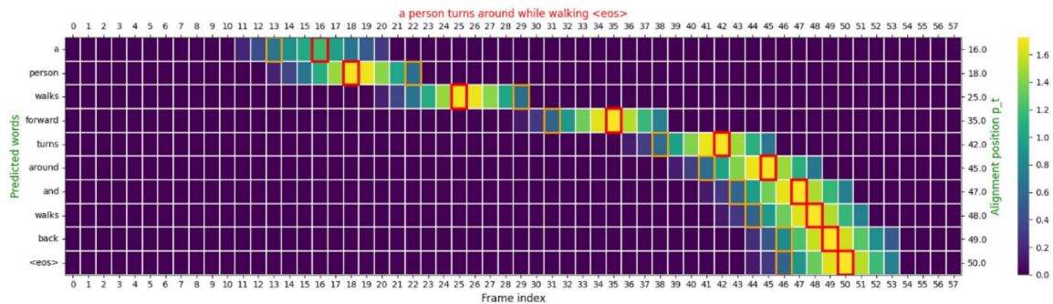
FIGURE 4.28: MLP[Local.rec.att]: Walk forward \llbracket 0, 30 \rrbracket , Turns around \llbracket 31, 40 \rrbracket and Walk backward \llbracket 41, 50 \rrbracket
