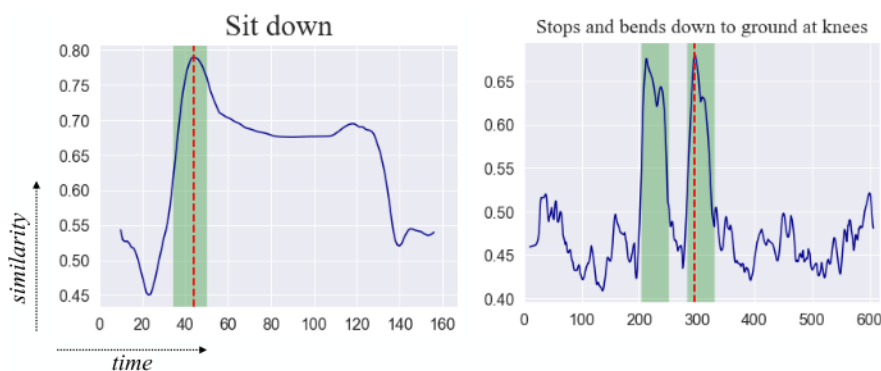
FIGURE 5.2: The ground-truth temporal span is denoted in green, the maximum similarity is marked with a dashed red line (Petrovich et al., 2023).
