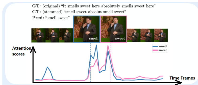
FIGURE 5.1: Attention scores evolution in frame time (Varol et al., 2021).
