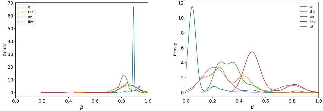
(a) Without gate supervision, decoder uses frequently motion information even for non-motion words ( \beta frequently high).
