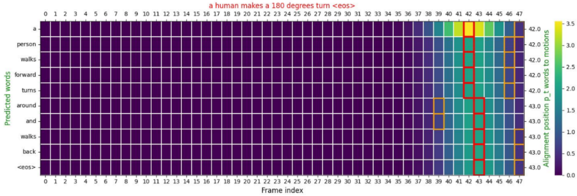
FIGURE 4.25: BiGRU[Loc.rec.att][Mask False]: Walk forward [[0, 21]] ; U-turn [[22, 34]] , Walk backward [[35, 47]]
