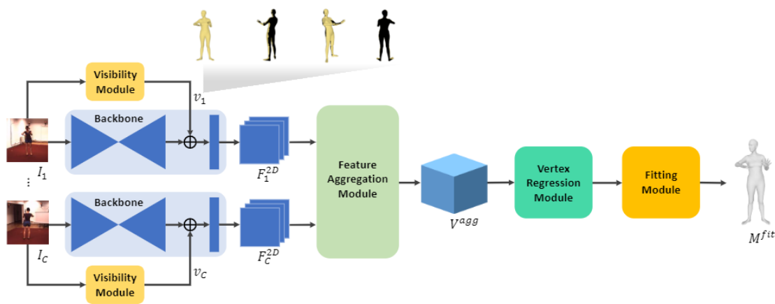
FIGURE 2.17: Overview : human-mesh based learnable triangulation (Chun et al., 2023).
