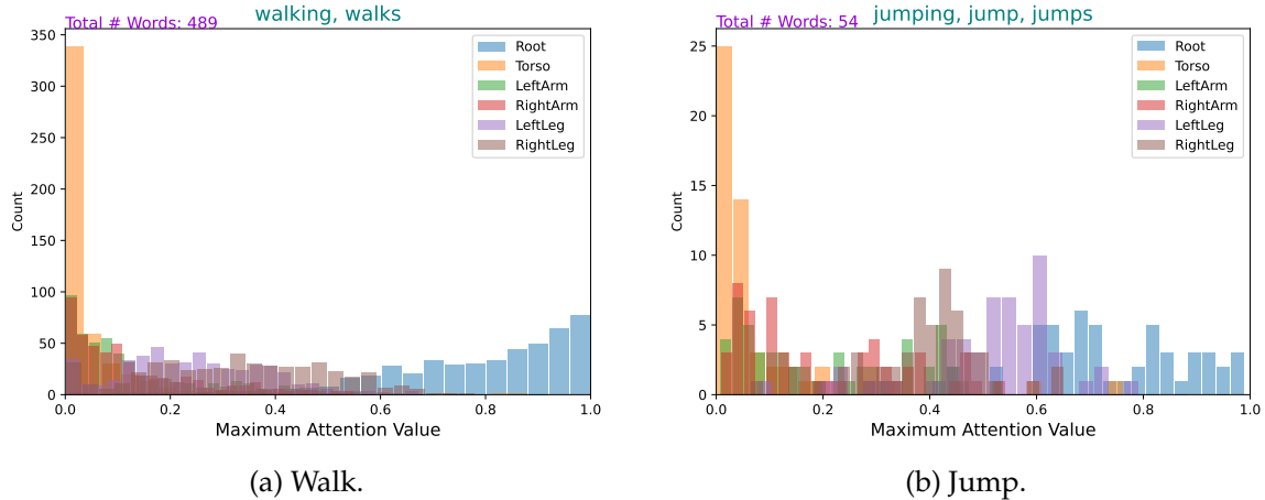
FIGURE 6.14: [KIT-(2,3)]: Body part distribution (spat+adapt).
