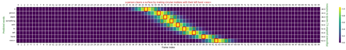
FIGURE 4.27: GRU[Loc.rec.att][Mask False]: wiping \llbracket 25, 56 \rrbracket
