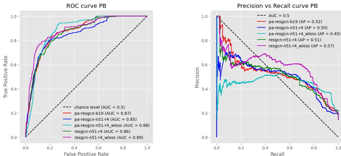
(a) ROC curves.
