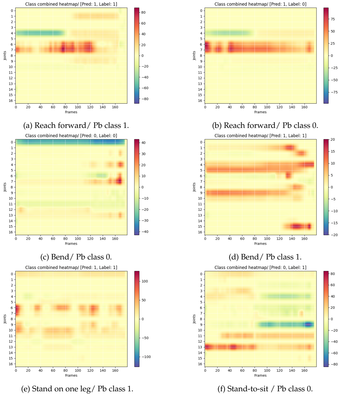
FIGURE 3.18: Combined CAM for ResGCN-N51 (Part 2).
