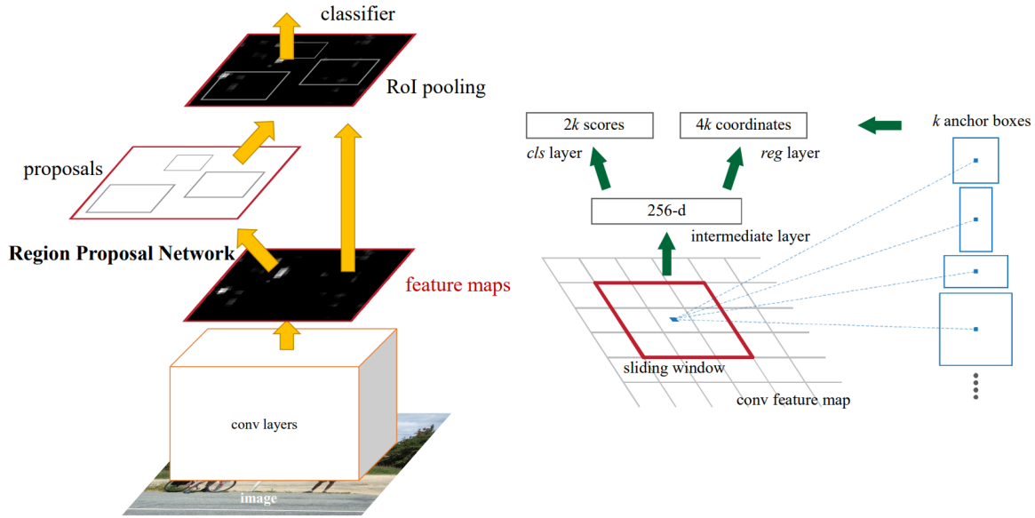
FIGURE 2.4: RPN Regional Proposal Network (RPN) (Ren et al., 2015).
