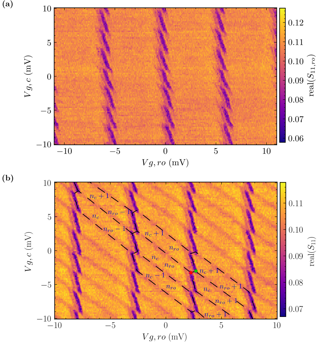
Figure 5.13: Charge stability diagrams for two different converter bias voltages: (a) V_c = 22 \mu\text{eV} (b) V_{ro} = 800 \mu\text{eV} . For low detector bias we detect only the tunneling through the readout SET, while for the bias at the superconducting gap (panel (b)), we see a response in the readout reflection when the tunneling through the converter SET is allowed. The distance in gate voltage between the two triple points (red and green dots in panel (b)) is used to measure the coupling capacitance between the two SETs.
