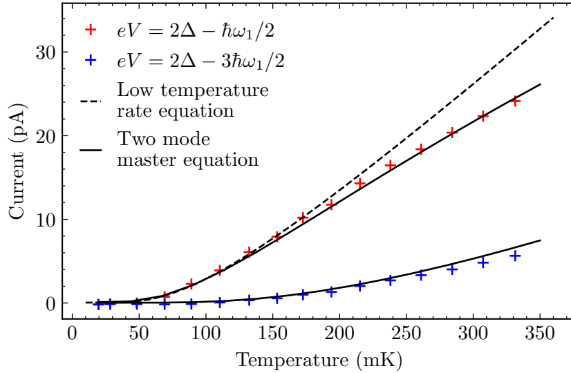
Figure 4.6: Current through the junction at bias voltage eV = 2\Delta - \hbar\omega_1/2 (red) and eV = 2\Delta - 3\hbar\omega_1/2 (blue). Dashed line represents the rate equation prediction (equation 4.3), while solid lines are master equation calculations taking the two lowest frequency modes from table 3.1. Dynes parameter is fixed to 10 neV in all calculations.
