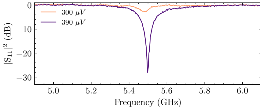
Figure 2.3: Two reflection spectra at different junction biases. Well below the superconducting gap ( V = 300 \mu\text{V} ) we see a small dip at resonance, while for V = 390 \mu\text{V} there is nearly perfect absorption at resonance — |S_{11}|^2 \approx -30 dB.
