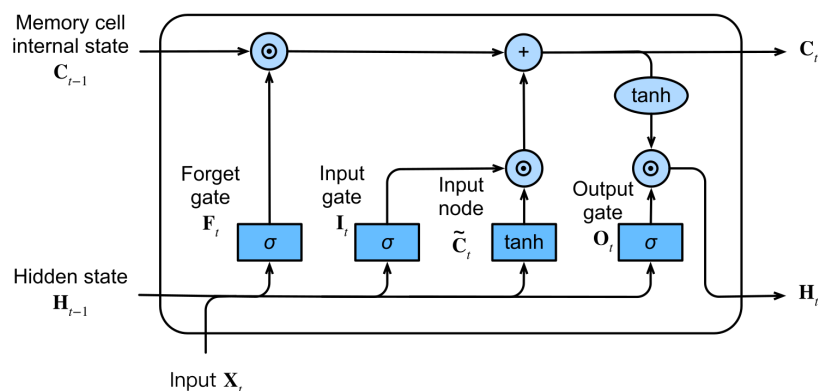
FIGURE 18 – Cellule LSTM
