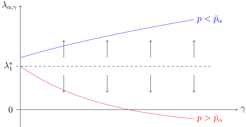
Figure 4.6: Illustration of Propositions 4.5.4 and 4.5.6.
