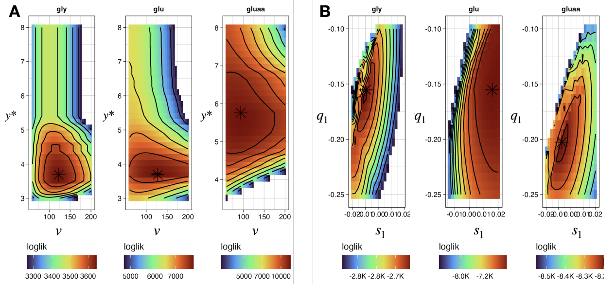
Figure 2.20: Log-likelihoods of the parameters of the SOS perturbed adder model. The MLE are marked *. A. Log-likelihood \ell_1 (2.27) of the division size observations as function of the critical mother length y^* and the concentration parameter v of the Beta mixture (2.19)-(2.20). B. Log-likelihood \ell_2 (2.28) of the added sizes at division as function of s_1 and q_1 .
