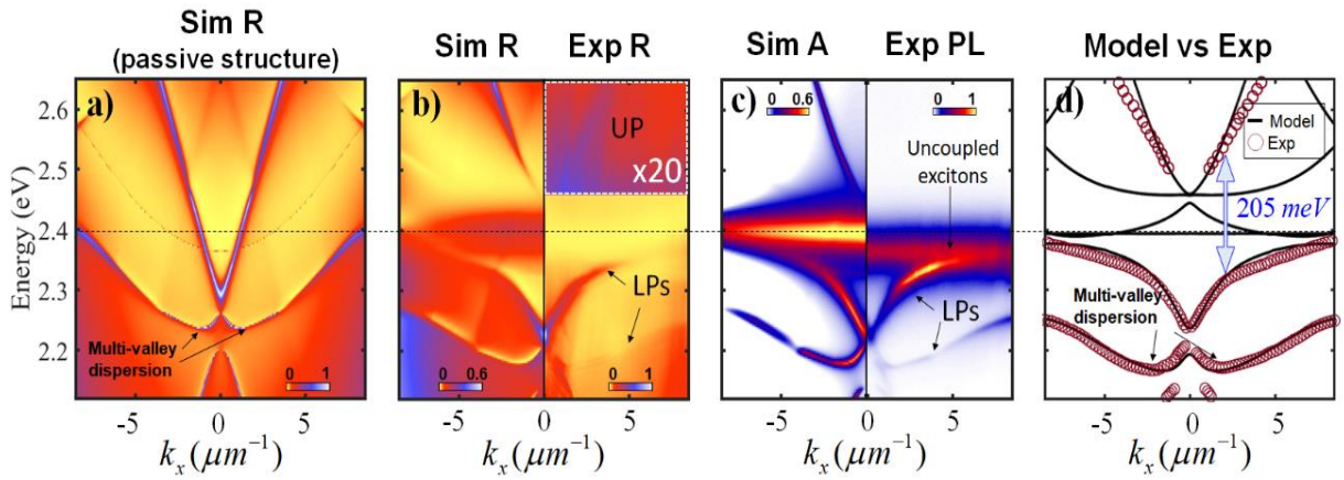
Figure 3.8. (a) Numerical simulations of the ARR for the passive structures. (b) Experimental results (right panel) and numerical simulations (left panel) of the ARR spectra for the active structures. (c) Experimental results of the ARPL response (right panel) compared to numerical simulations of the angular-resolved absorption by RCWA (left panel) for the active structures. (d) Numerical solution of photonic crystal polariton dispersions from a quantum model of radiation-matter interaction, compared to experimental results extracted from ARR measurements. The black dash line represents the energy of the PEPI excitonic resonance.
