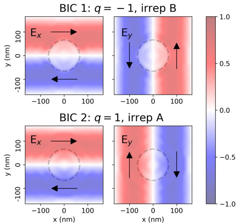
Figure C1. Symmetry properties of \text{BIC}_1 and \text{BIC}_2 .
