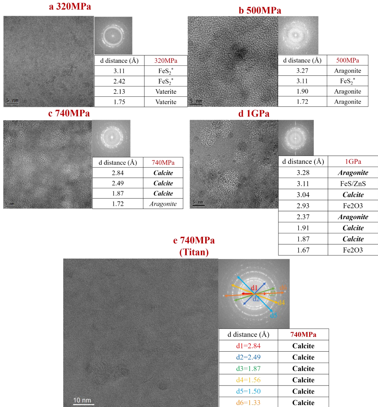
Fig. 3.11 TEM diffraction mode on cross-sections and d-distance measurements at 320MPa (a), 500MPa (b), 740MPa (c), 1GPa (d) and 740MPa verified by Titan microscope (e) [6-8]
