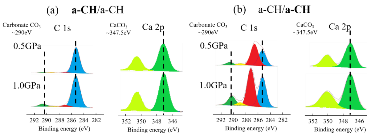
Fig. 5.15 XPS high resolution spectra of C 1s and Ca 2p on the a-C:H ball (a) and on the a-C:H disk (b)
