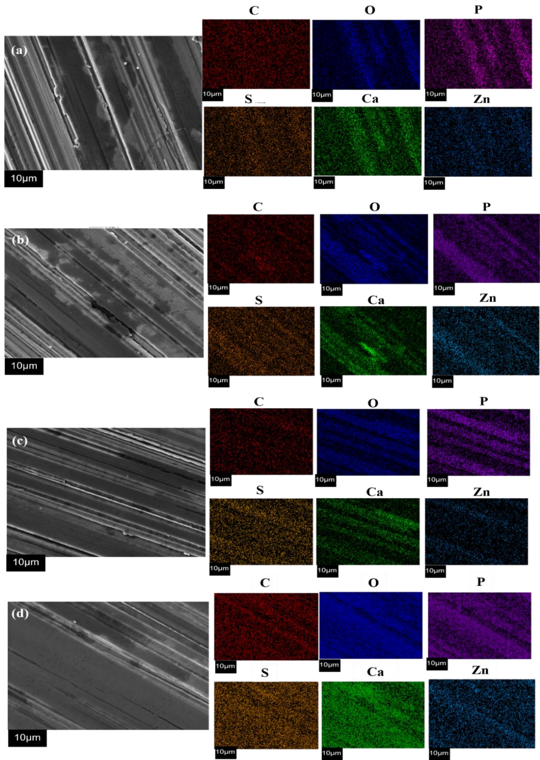
Fig. 3.7 SEM images of rings for steel ring (not polished)/a-C:H disk at 320MPa (a), 500MPa (b), 740MPa (c), 1GPa (d) and the corresponding EDS mapping results of C, O, P, S, Ca and Zn.
