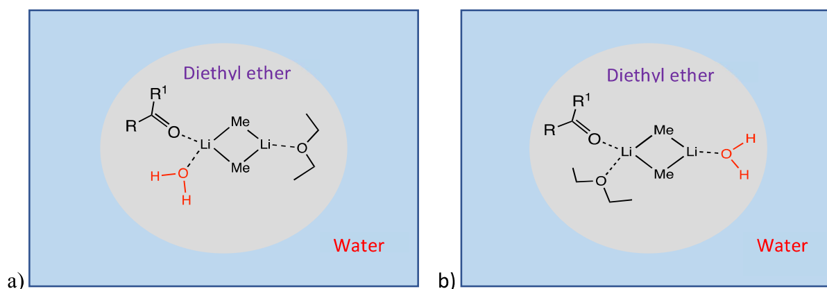
Fig. 5.2: oil—water droplet model with reactants in the diethyl ether phase (oil) surrounded by water surface: a) diffused water coordinated to Li b b) diffused water coordinated to Li nb
