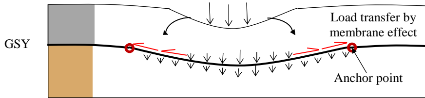
Figure 2-5: Tensioned membrane effect
