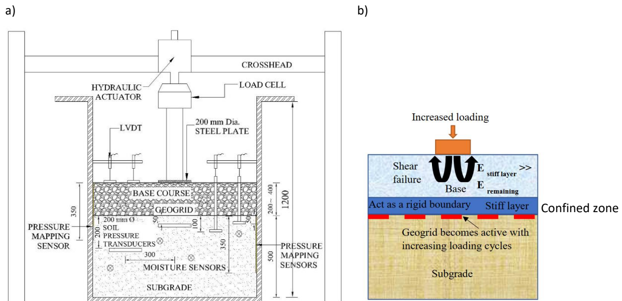
Figure 2-15: Jayalath et al. (2021): a) Schematic diagram of the experimental setup (dimension in mm); b) Rigid boundary effect
