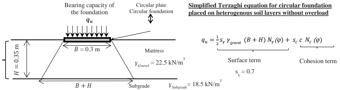
Figure 5-15: Analytical calculation of the bearing capacity of a plate placed on a superficial granular layer above a subgrade soil using the simplified Terzaghi Equation
