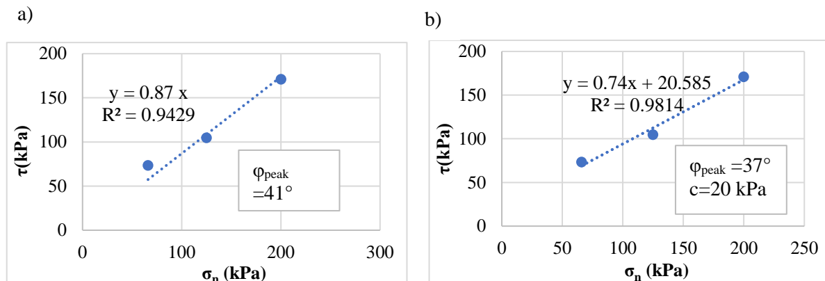
Figure 3-12: Maximum shear versus the normal stress of the aggregate-aggregate interface
