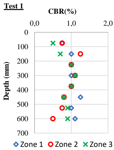
Figure 4-3: CBR profiles of three different zones within the subgrade layer of Test 1
