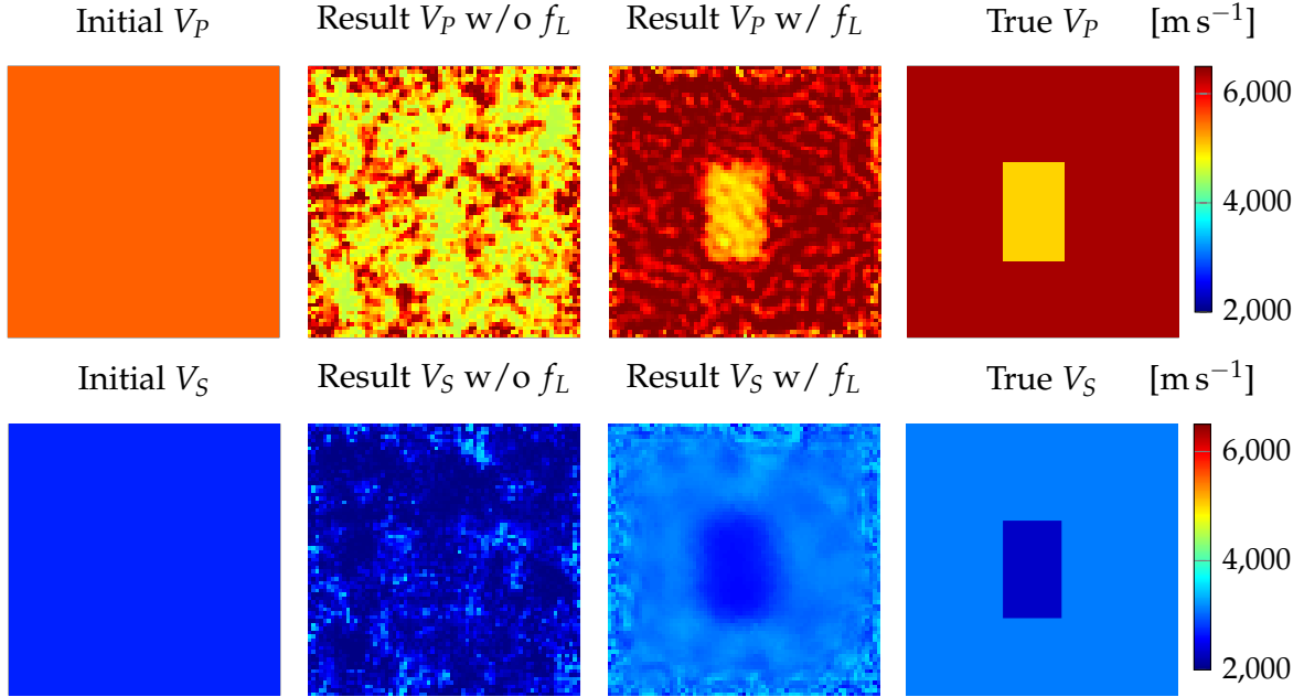
Figure V.16: Inversion on elastic medium (no viscosity) with and without the use of complex (Laplace) frequencies. V_P and V_S final inversion results for the frequencies 100 kHz to 900 kHz with a step of 100 kHz with the initial model V_P = 5500 \text{ m s}^{-1} and V_S = 3100 \text{ m s}^{-1} . Results without (w/o) and with (w/) the use of Laplace frequencies f_L = [400;200;100] kHz. There is no viscous attenuation in the true model.
