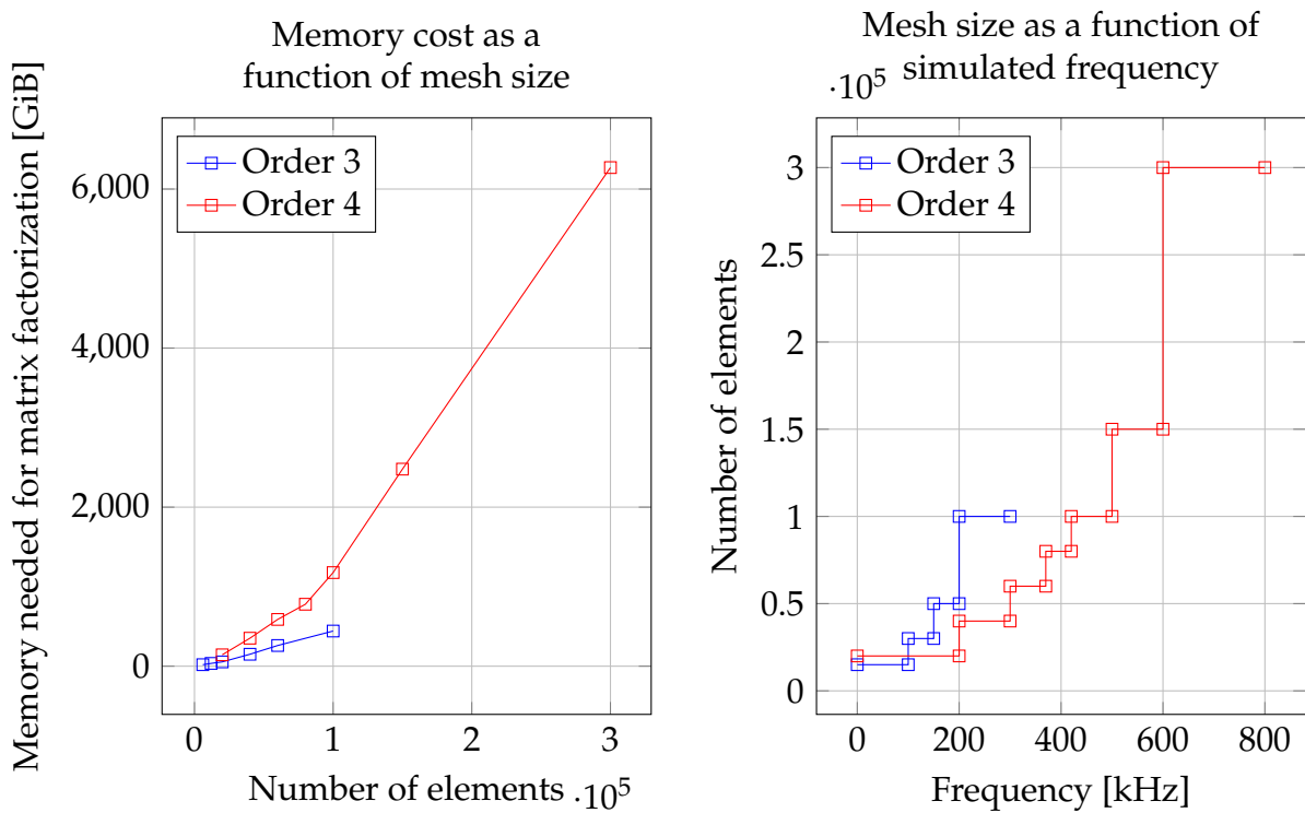
Figure III.7: [left] Computational cost with respect to the number of elements in the mesh for HDG simulation, with cells of order 3 or 4. [right] Used number of elements of order 3 or 4 for a simulation in a 7 cm x 7 cm x 7 cm cube with respect to simulated frequency. The wavelength of the S-waves is 1 cm at 310 kHz.
