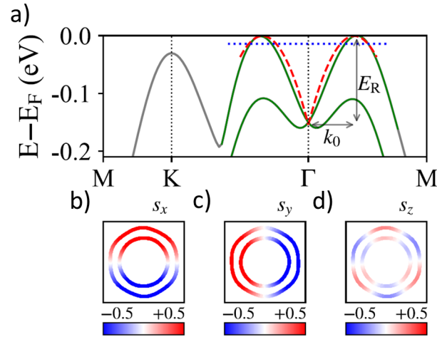
Figure 4.2: a) Zoom-in plot of the two highest valence bands around \Gamma point. The top one is fitted with a generalized Rashba Hamiltonian (red dashed line). b-d) at a constant energy (highlighted by the blue dotted line), spin components of the band [5].
