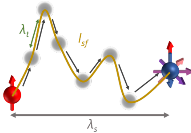
Figure 1.4: A representation of \lambda_s and \lambda_{sf} showing the electron spin is flipping after a certain distance into a material.
