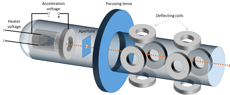
Figure 2.4: E-beam generation by a RHEED electron gun and directing it towards the growing film using magnetic deflectors. Adapted from Hasegawa et al [75].
