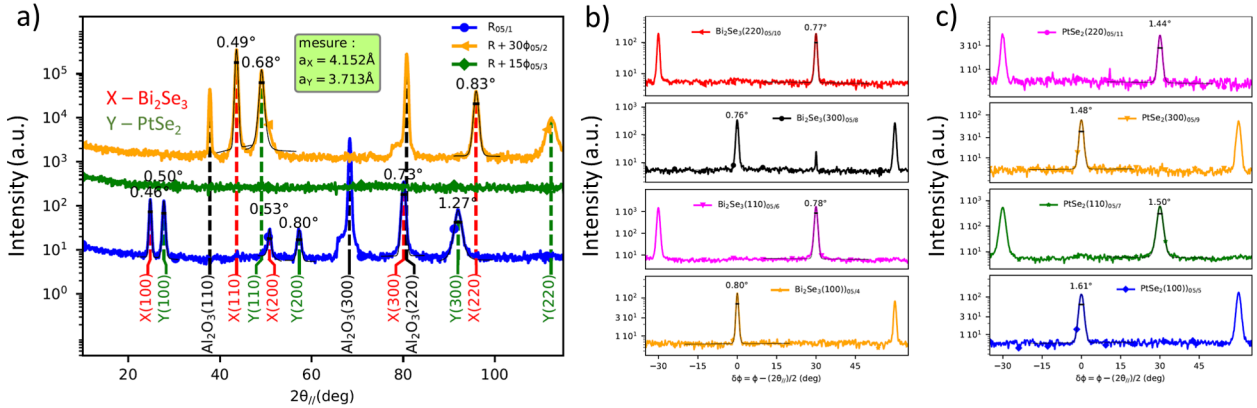
Figure 5.8: In-plane XRD of a) 5 ML \text{PtSe}_2 /10 ML \text{Bi}_2\text{Se}_3 on sapphire and b) and c) azimuthal scans of \text{Bi}_2\text{Se}_3 and \text{PtSe}_2 , respectively, showing very little mosaic spread. This high anisotropy is attributed to the strong interaction with the substrate that does not give much degree of freedom for the growing grains to rotate.
