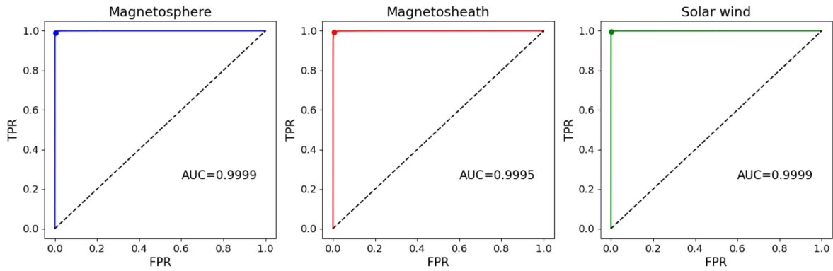
Figure 2.11: The Receiver Operator Curve (ROC) curve for the THEMIS model. The panels from left to right show the ROC curve for the magnetosphere, magnetosheath, and solar wind classifications. The colored point on the curve corresponds to the true positive rate and false positive rate achieved with a decision threshold set at 0.5.
