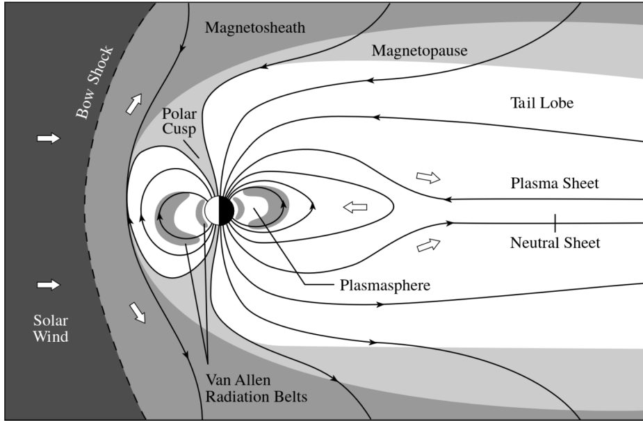
Figure 1.5: Schematic of near-Earth plasma environment in the meridional plane. Figure from Lang [2011].
