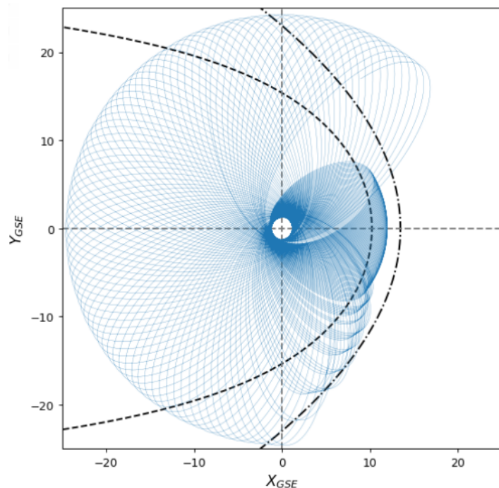
Figure 2.7: Orbit of the MMS1 spacecraft in the equatorial plane between November 26th, 2016 and November 25th, 2017. The dashed and dash-dotted black lines correspond to the magnetopause and bow shock, respectively.
