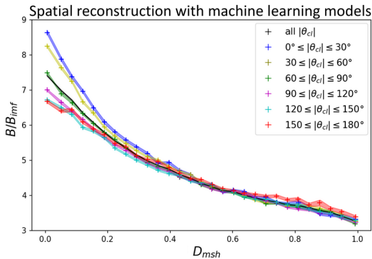
Figure 2.19: Spatial reconstruction of the magnetic pileup, for different range of IMF clock angles, in the subsolar magnetosheath as function of the relative distance ( D_{msh} ) to the magnetopause and bow shock obtained with the machine learning models. The magnetopause is located at D_{msh}=0 , while the bow shock is at D_{msh}=1 .
