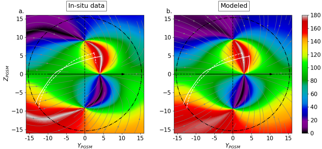
Figure 5.9: Magnetic shear maps at low IMF cone angle. Subsets |\theta_{co}| \leq 12.5^\circ and |\psi| = 0^\circ \pm 2.5^\circ with \theta_{cl} = 90^\circ . Panels a and b correspond to the magnetic shear angle maps made using only in-situ measurements and magnetic field models [Kobel and Fluckiger, 1994; Tsyganenko and Stern, 1996], respectively. The magnetic shear map on panel b correspond to the one presented in Trattner et al. [2012a] (Figure4) on the 22 Mars 1996 at 02:40 UT. The grey arrowed lines represent in the panels a and b represent magnetic field lines of the observed and modeled magnetosheath draping, respectively. The solid and dashed white lines maximize the observed and modeled magnetic shear (MSL), respectively. ( Y_{PGSM}Z_{PGSM} ) plane. The magnetopause terminator is represented by the dashed-dotted circle.
