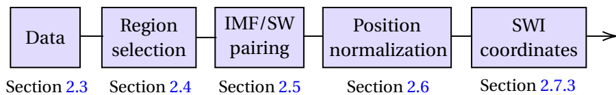
Figure 4.1: Overview of the global methodology detailed in Chapter 2.
