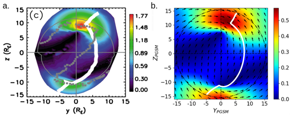
Figure 3: The color maps correspond to the MHD scaling law for the local reconnection rate [Cassak and Shay, 2007] from a simulation [Komar et al., 2015] in panel a and from in-situ data in panel b. In panel a, the gray line represents the line that globally maximizes the reconnection rate, and the white line corresponds to the magnetic separator obtained in the simulation. The white line in panel b corresponds to the X-line predicted by the new X-line model.
