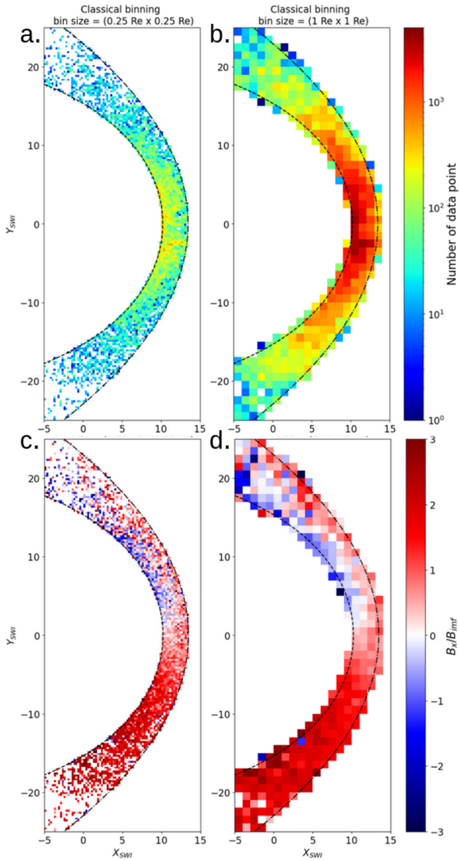
Figure 2.27: Count of the number of point per bin (panels a and b ) and distributions of the B_x/B_{imf} (panels c and d ) in the equatorial plane ( |Z_{SWI}| \leq 0.5 \text{ Re} ) for measurements falling within |\theta_{co}|=25^\circ \pm 5^\circ using the classical binning method for 0.25 Re (panels a and c ) and 1 Re (panels b and d ) square bins.
