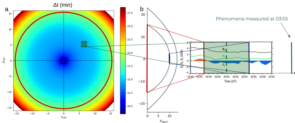
Figure 6: Panel a corresponds to the time it takes for the IMF to propagate from the bow shock to the magnetopause in minutes, determined by integrating the in-situ velocity measurements. The red and blue circles indicate the terminator and the vicinity to the subsolar point of the magnetopause, respectively. The green cross represents the location of a considered event at the magnetopause. Panel b shows a schematic illustrating the attribution of different IMF orientations to the various positions of the magnetopause surface for the event measured at 03:05 UT (green vertical line). The IMF orientation measured at the blue and red vertical lines are attributed to subsolar region and the terminator of the magnetopause, respectively. The green dashed vertical line corresponds to the IMF condition for the considered event. The green area represents all of the IMF orientation found on the dayside magnetopause surface.
