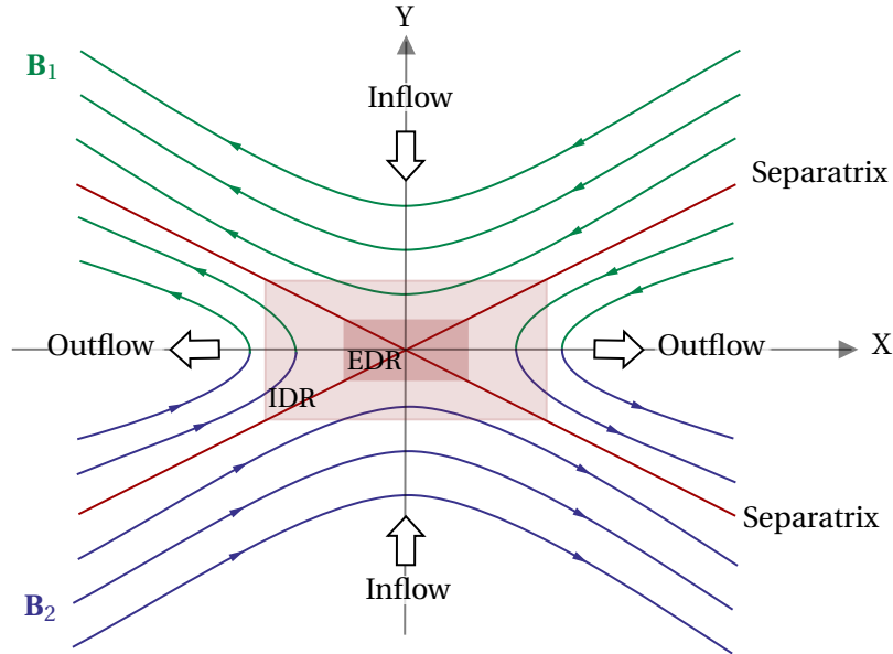
Figure 1.7: Schematic illustration of magnetic reconnection in the reconnecting plane (XY). The green ( B_1 ) and blue ( B_2 ) lines represent the upstream magnetic field lines that will undergo reconnection, while the green-blue bicolor lines correspond to the magnetotoc lines that have already reconnected. The red lines are the separatrices. The arrows indicate the plasma inflow and outflow. The lighter and darker red rectangles represent the IDR and EDR.
