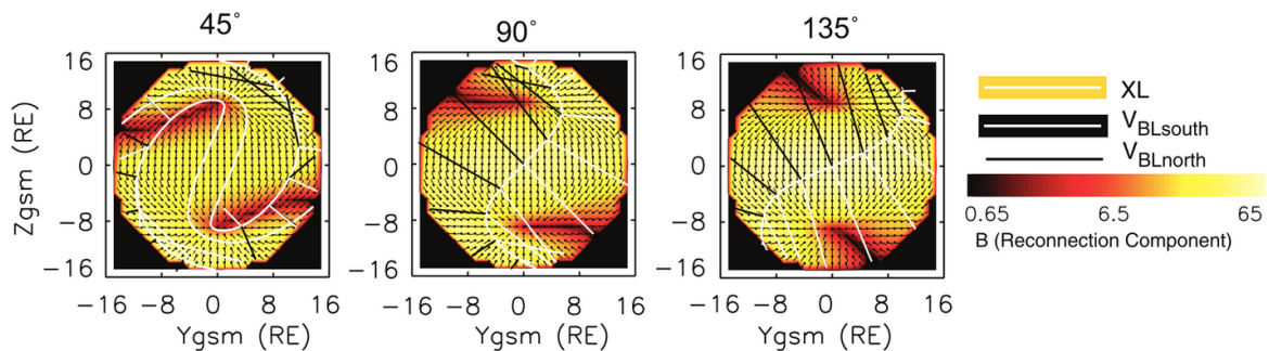
Figure 1.15: The color coded map represents reconnecting component magnitude on the dayside magnetopause, as view from the sun, for IMF clock angle of 45°, 90°, and 135°. The curved white lines that correspond to the X-lines predicted by Moore et al. [2002]'s model. The straight black and white lines represent the boundary layer flow rooted in the northern and southern hemispheres, respectively. Figure adapted from Moore et al. [2002].
