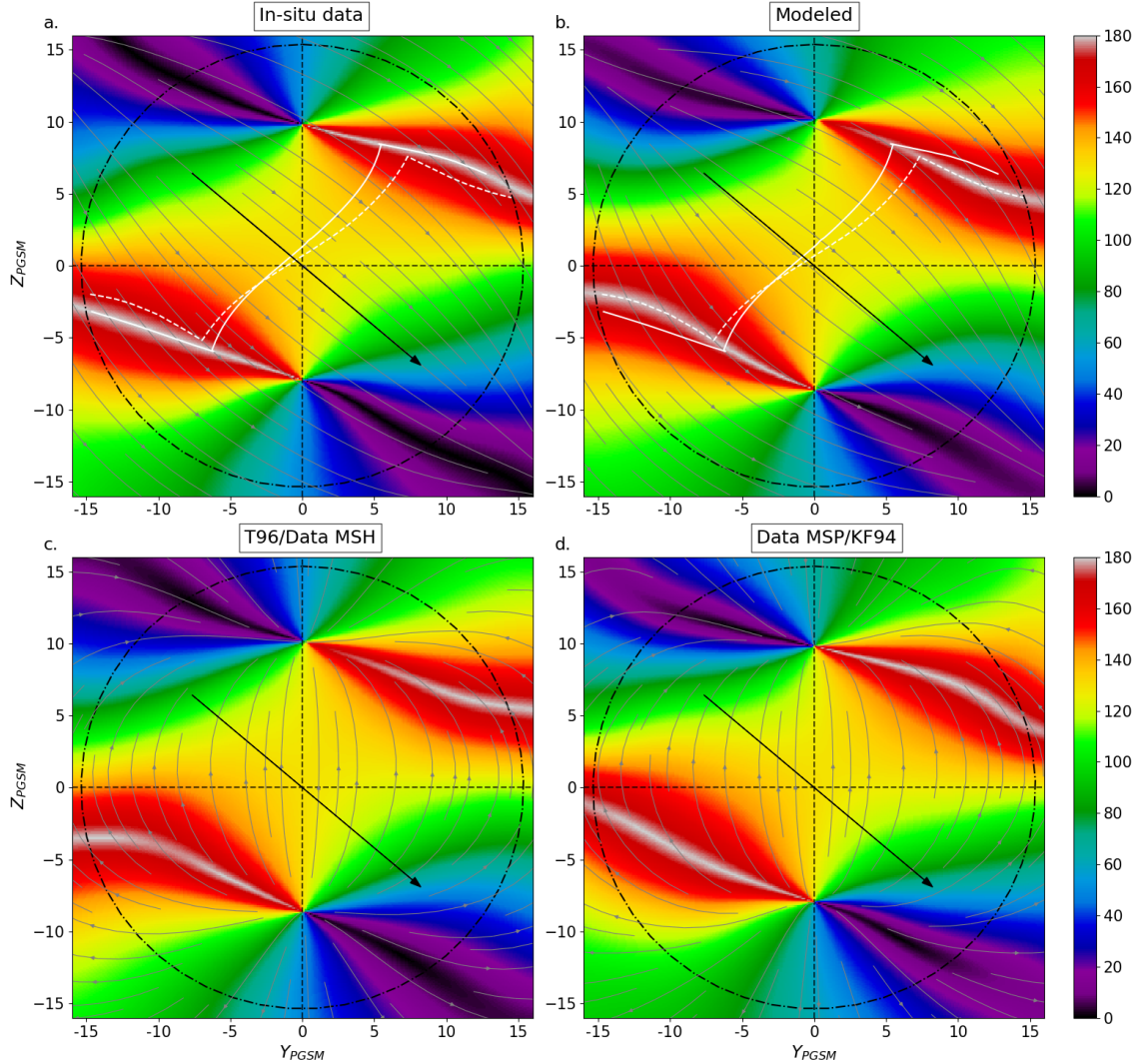
Figure 5.6: Magnetic shear maps at large IMF cone angle. Panels a and b correspond to the magnetic shear angle maps using only in-situ measurements and magnetic field models [Kobel and Fluckiger, 1994; Tsyganenko and Stern, 1996], respectively. The magnetic shear map on panel b correspond to the one presented in Trattner et al. [2021] (Figure13) on 20 September 1997 at 07:34 UT. The map in panel c is made with the T96 model and the magnetosheath in-situ measurements. The map in panel d is made with the magnetosphere in-situ measurements and the KF94 model. The subset of in-situ magnetosheath measurements used in panels a and c is 76^\circ \leq |\theta_{col}| \leq 86^\circ and turned to an IMF clock angle of 130^\circ . The subset of in-situ magnetosphere measurements used in panels a and d is |\psi| = 6.6^\circ \pm 2.5^\circ . The value of dipole tilt of modeled magnetospheric magnetic field (T96) used in the panels b and c is -6.6^\circ . The modeled magnetosheath magnetic field (KF94) in the panels b and d is made with (B_{x_{imf}}, B_{y_{imf}}, B_{z_{imf}}) = (-0.7, 3.8, -3.2) . The grey arrowed lines in the panels a and b (resp. c and d) represent magnetic field lines of the observed and modeled magnetosheath (resp. magnetosphere), respectively. The solid and dashed white lines maximize the observed and modeled magnetic shear, respectively. The black arrows correspond to IMF orientation in the (Y_{PGSM}, Z_{PGSM}) plane. The magnetopause terminator is represented by the dashed-dotted circle.
