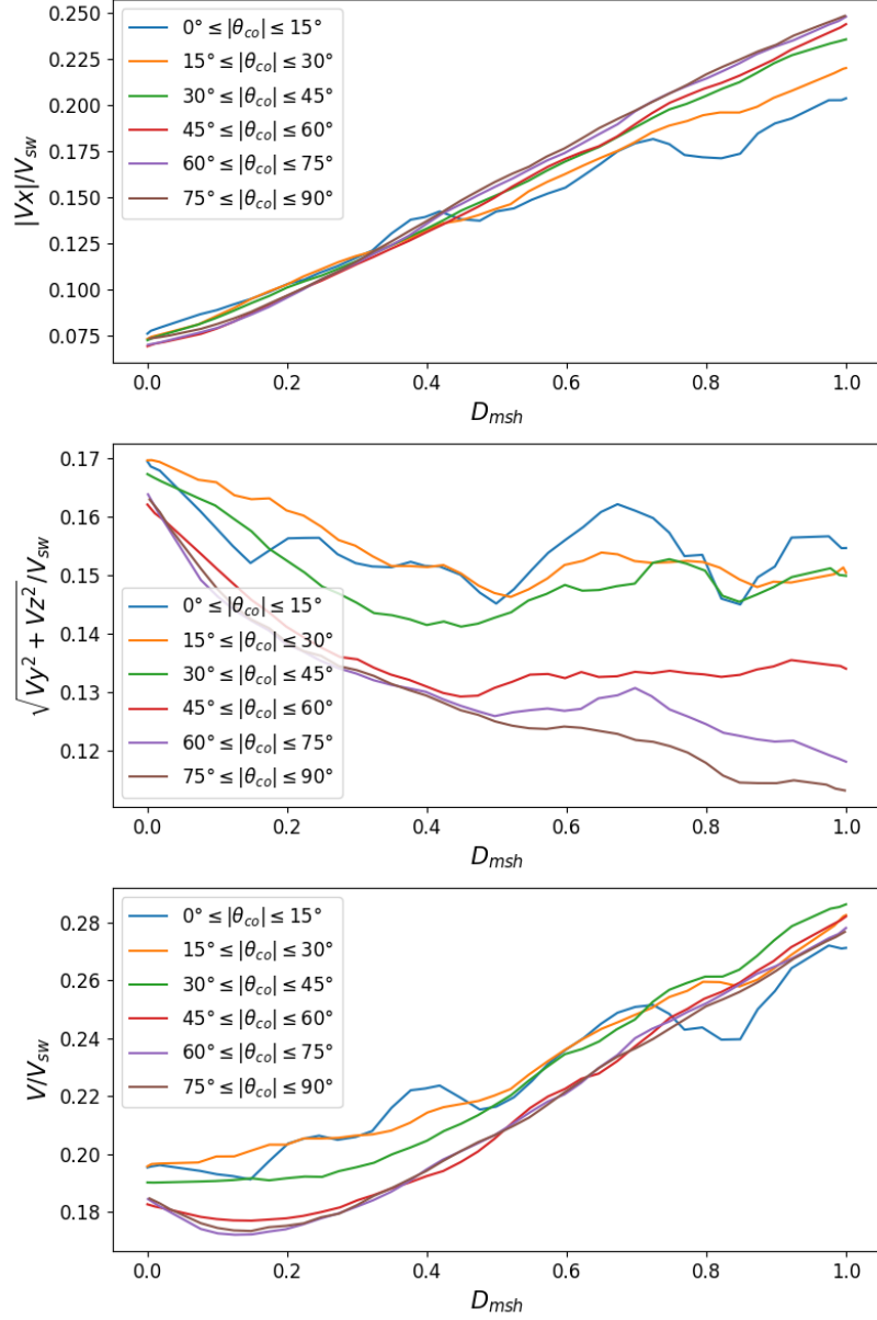
Figure 4.4: Velocity profiles in the subsolar magnetosheath ( \sqrt{Y^2 + Z^2} \leq 5 R_e ) normalized by the solar wind velocity as a function of the position in the magnetosheath D_{msh} relative to the magnetopause and bow shock. From top to bottom panel is represented: V_x/V_{sw} , V_{yz} = \sqrt{V_y^2 + V_z^2}/V_{sw} and V/V_{sw} . The magnetopause and bow shock are positioned at D_{msh}=0 and D_{msh}=1 , respectively. The different colored lines represent the velocity profiles for different absolute value of IMF cone angles ( |\theta_{co}| ).
