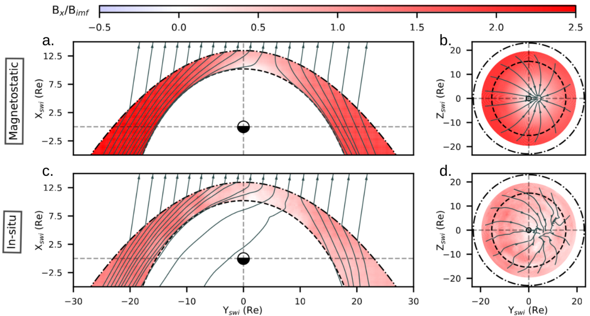
Figure 3.9: Small IMF cone angle draping corresponding to the subset of measurements falling within 0^\circ \leq |\theta_{co}| \leq 12.5^\circ . Panels (a, b) and (c, d) correspond respectively to magnetostatic Kobel and Fluckiger [1994] and in-situ data magnetic field. The color maps correspond to B_x/B_{imf} . The grey arrowed lines correspond to the magnetic field lines integrated in 3D (see section 3.2.1). Panels a and c correspond to the data close to the Z_{SWI} = 0 plane. Panels b and d correspond to the data close to the magnetopause.
