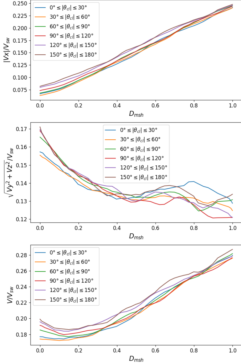
Figure 4.6: Velocity profiles in the subsolar magnetosheath ( \sqrt{Y^2 + Z^2} \leq 5 R_e ) normalized by the solar wind velocity as a function of the position in the magnetosheath D_{msh} relative to the magnetopause and bow shock. From top to bottom panel is represented: V_x/V_{sw} , V_{yz} = \sqrt{V_y^2 + V_z^2}/V_{sw} and V/V_{sw} . The magnetopause and bow shock are positioned at D_{msh}=0 and D_{msh}=1 , respectively. The different colored lines represent the velocity profiles for different absolute value of IMF clock angles ( |\theta_{cl}| ).
