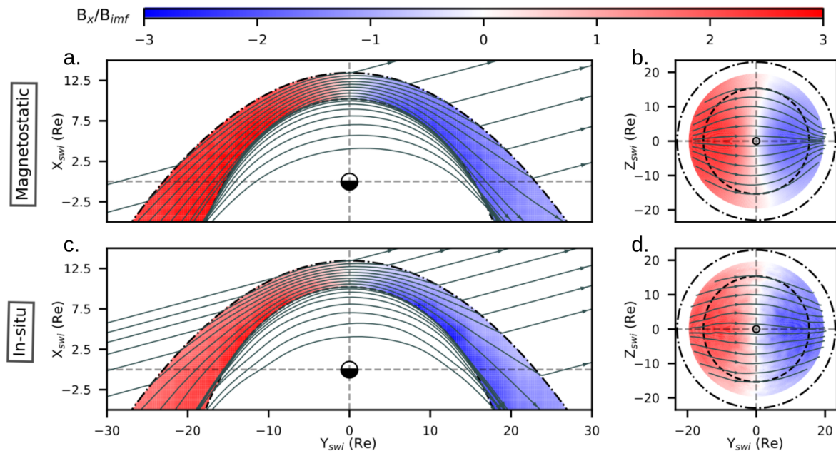
Figure 3.3: Large IMF cone angle draping corresponding to the subset of measurements falling within 70^\circ \leq |\theta_{co}| \leq 80^\circ . Panels (a, b) and (c, d) correspond respectively to magnetostatic Kobel and Fluckiger [1994] and in-situ data magnetic field. The color maps correspond to B_x/B_{imf} . The grey arrowed lines correspond to the magnetic field lines integrated in 3D (see section 3.2.1). Panels a and c correspond to the data close to the Z_{SWI} = 0 plane. Panels b and d correspond to the data close to the magnetopause.
