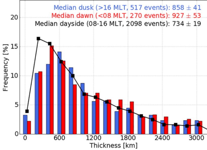
Figure 5.2: Histograms of the thickness in units of kilometers for the dayside, dawn and dusk magnetopause flanks. The Magnetic Local Time (MLT) coordinates correspond to the hour angle formed by the meridional plane that contain the subsolar point with the meridional plane of the considered position. Figure adapted from Haaland et al. [2020] .
