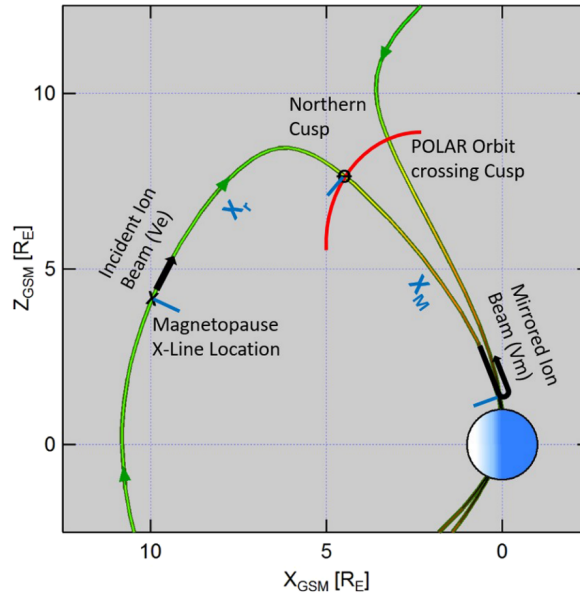
Figure 1.25: Schematic diagram of ion injection into the northern cusp from newly reconnected field lines and those reflected at low altitude. V_e and V_m correspond to the incident and mirrored velocity, respectively. X_r (resp. X_m ) corresponds to the distance between the Polar spacecraft and the X-line location (resp. the ionospheric mirror point). Figure from Trattner et al. [2021b] .
