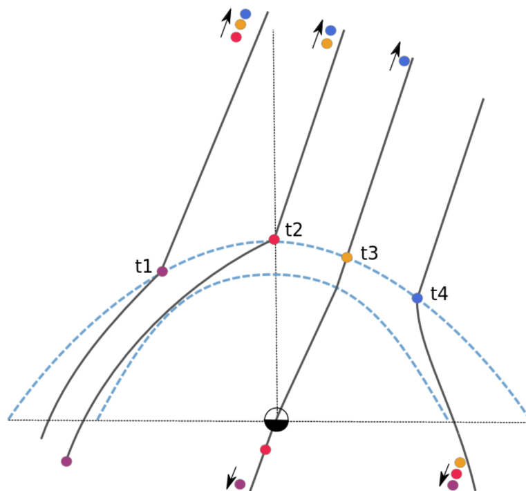
Figure 3.11: Schematic of the draping mechanism for the low IMF cone angle regime. t1 to t4 represent the arrival time at the bow shock of the different fluid elements (purple, red, orange and blue points) connected by the same magnetic field line.
