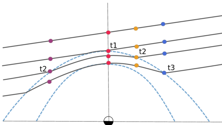
Figure 3.5: Schematic of the draping mechanism for the large cone angle regime. t_1 to t_3 represent the arrival time at the bow shock of the different fluid elements (purple, red, orange and blue points) connected by the same magnetic field line.
