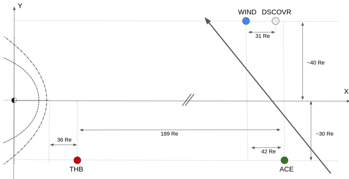
Figure 4: Configuration of the THEMIS-B , ACE, Wind, and DSCOVR spacecraft within the interplanetary medium on January 7, 2016, at approximately 09:30 UT. The gray arrow represents the IMF in the ecliptic plane.
