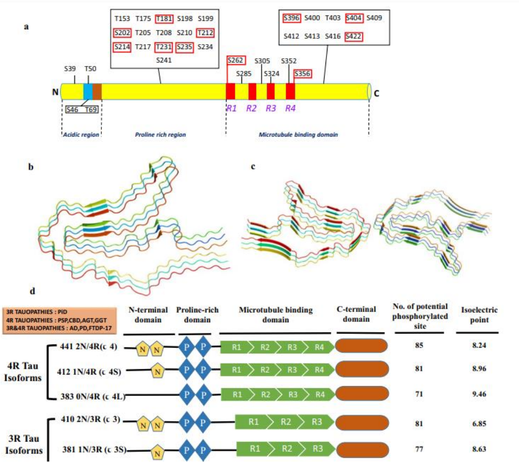
Figure 28. Tau protein.
