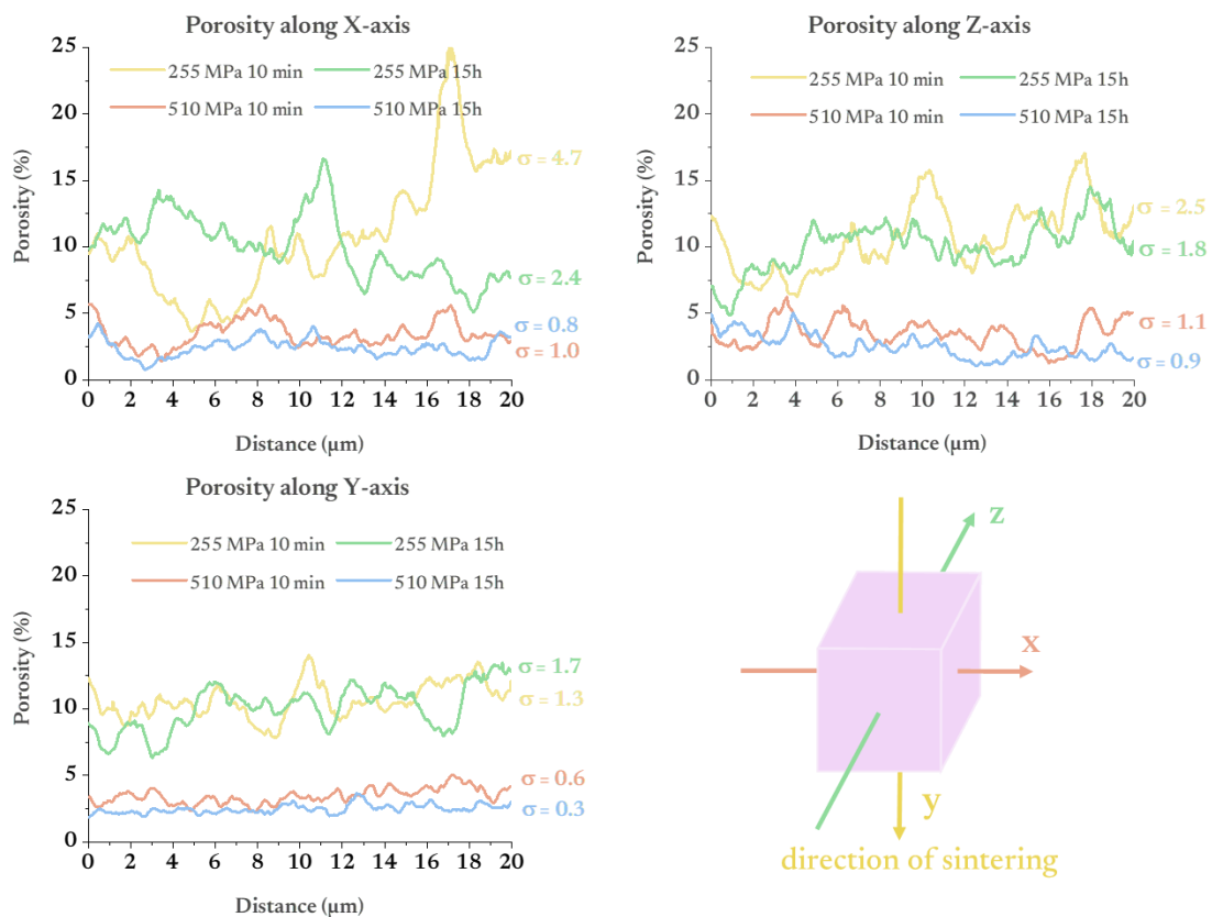
Figure 45: Porosity per slice along the three axes with the standard deviation of porosity, Y axis toward the centre (same axis as the applied pressure), X and Z axes toward the edge of the pellet.
