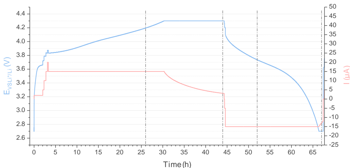
Figure 85: Galvanostatic cycling at ca. C/60 rate between 2.7 and 4.3 V vs. Li + /Li with a potential hold until one-fifth of the initial current (15 μA) is reached. The dashed grey lines indicate the time the images were acquired.
