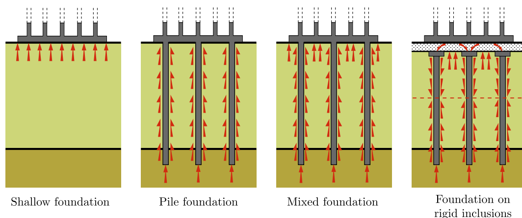
Fig. 1.1. Illustration of the load transfer mechanism in various foundation types
