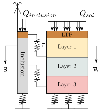
Fig. 5.18. Two-phase soil-inclusion elementary cell model
