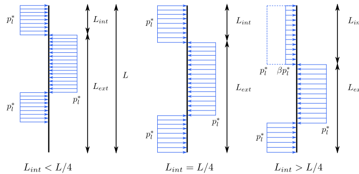
Fig. 8.17. Distribution of lateral pressure for limit equilibrium model (MEL I)
