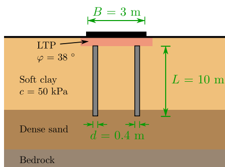
Fig. 11.25. Foundation configuration used in pseudo-static study
