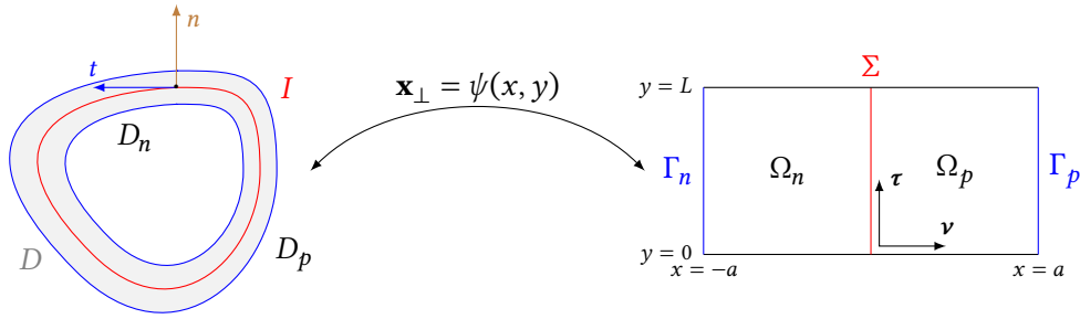
Figure 4.1: [Left] The tubular neighborhood D of I . [Right] The domain \Omega = (-a, a) \times (0, L) . [Center] The transform \psi : \bar{\Omega} \rightarrow \bar{D} with \psi(\Sigma) = I , \psi(\Omega_{p,n}) = D_{p,n} and \psi(\Gamma_{p,n}) = \partial D_{p,n} \setminus I .
