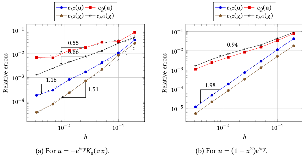
Figure 7.11: Relative errors for the formulation with a discretized jump with \mathcal{F}_h^{\Omega, unstr} and \omega = 1 .
