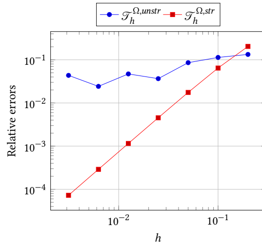
Figure 7.8: Relative error e_{L^2}(\mathbf{u}) for the first simplified formulation with structured meshes \mathcal{T}_h^{\Omega,str} and unstructured meshes \mathcal{T}_h^{\Omega,unstr} , and u = -K_0(\pi x)e^{i\pi y} .
