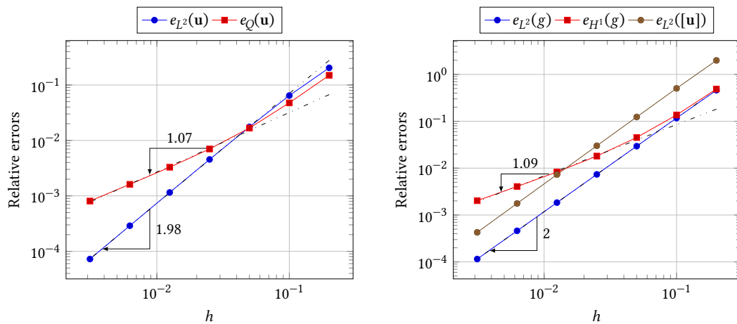
Figure 7.9: Relative errors for the simplified variational formulation with \mathcal{T}_h^{\Omega,str} , and u = -K_0(\pi x)e^{i\pi y} .
