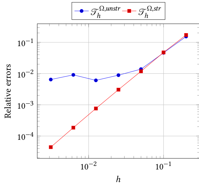
Figure 7.4: Influence of structuring \mathcal{T}_h^{\Omega} on the stability of the method.
