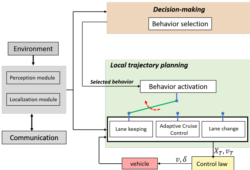
Figure 3.1. Multi-Controller Architecture
