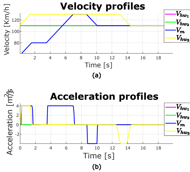
Figure 5.12. The vehicles' velocity and acceleration profiles
