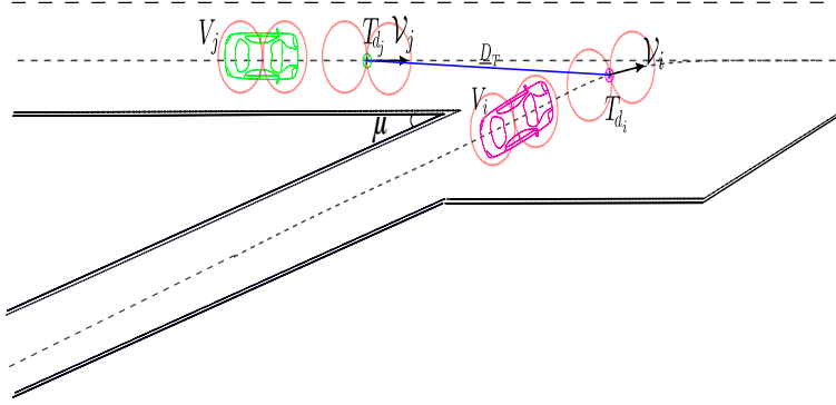
Figure 4.2. Illustration of the merging scenario where the minimum inter-distance \underline{D}_T is depicted
