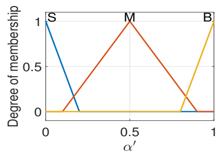
Figure 2.6 – Fuzzy sets - output
