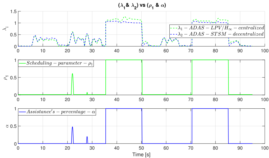
Figure 4.29 – \lambda_i vs \rho and \alpha - Scenario 1
