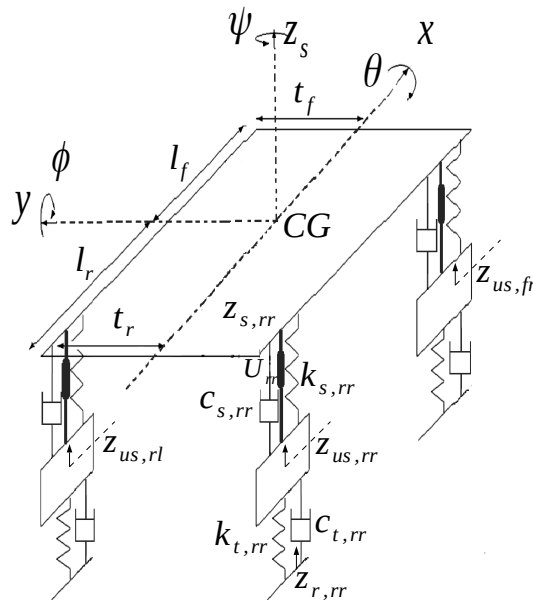
Figure 1.3 – Full vehicle vertical model [Chokor, 2019]
