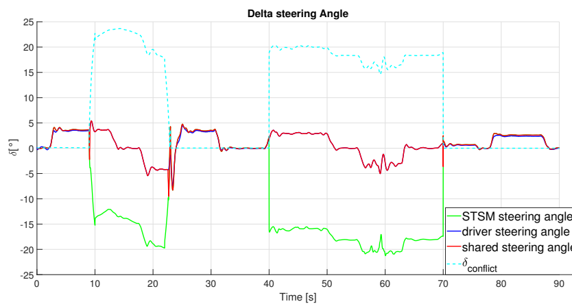
Figure 2.19 – The different steering wheel angles - case 1, on SCANeR Studio simulator
