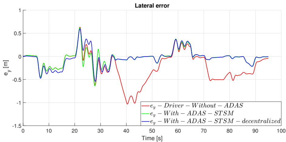
Figure 4.54 – STSM controllers - e_y comparison
