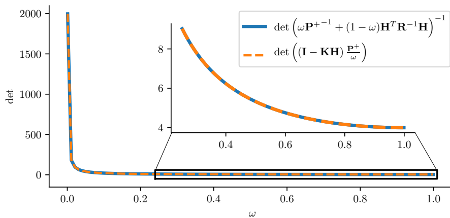
Figure 2.14: Curve of the fused covariance matrix determinant for \omega between from 0 to 1 in the case of a partial measurement. The region between 0.25 and 1 is zoomed in.
